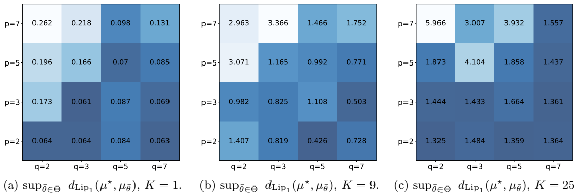
Figure 3: Influence of the generator’s depth p and the discriminator’s depth q on the maximal Wasserstein distance \sup_{\bar{\theta} \in \bar{\Theta}} d_{\text{Lip}_1}(\mu^*, \mu_{\bar{\theta}}) .
