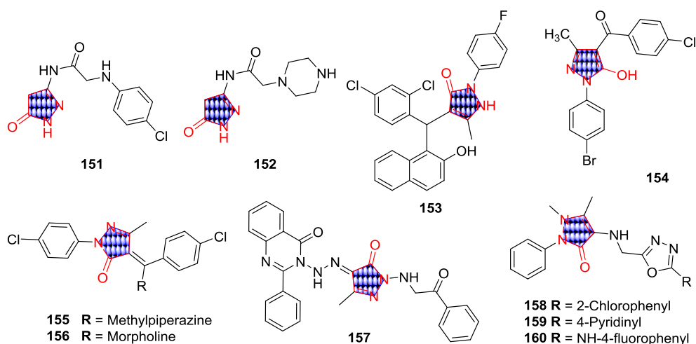
Figure 15. Pyrazolones with antitubercular activity.
