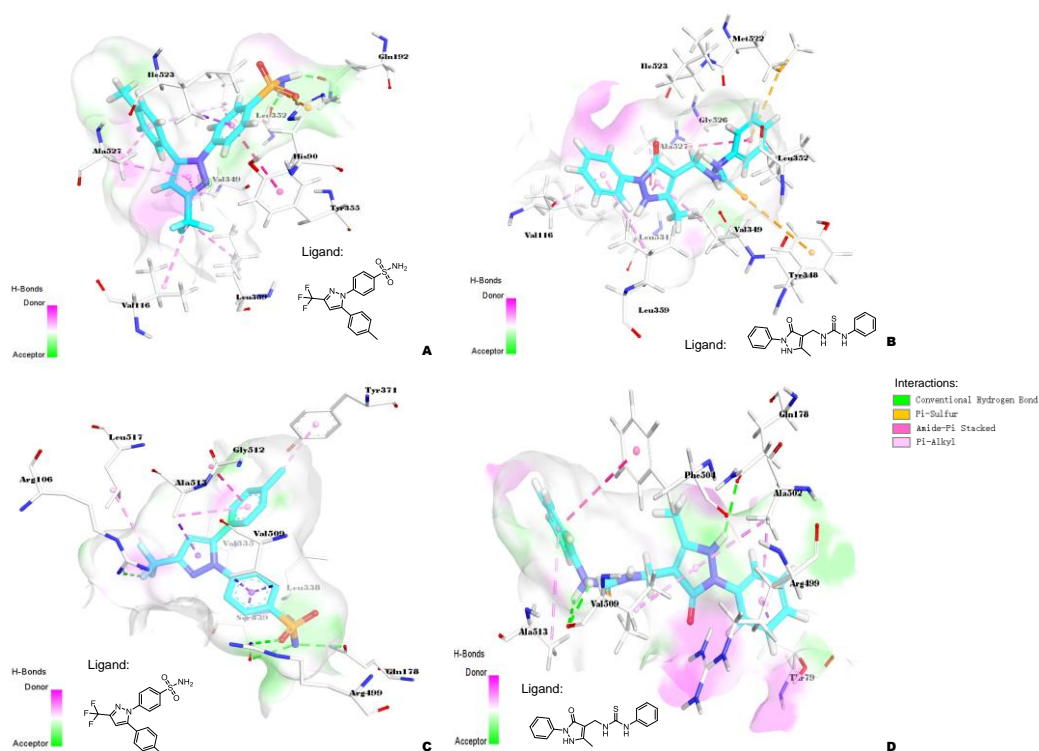
Figure 12. Ligand-protein interactions of celecoxib (A) and pyrazolone derivative 131 (B) with the active site of COX-1 (PDB ID: 3KK6), celecoxib (C) and pyrazolone derivative 131 (D) with the active site of COX-2 (PDB ID: SLN1) accomplished by Discovery Studio 2019.
