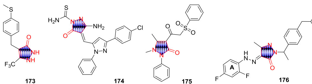
Figure 18. Pyrazolones as antihyperglycemic agents.
