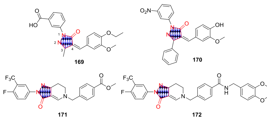
Figure 17. Pyrazolones as lipid-lowering agents.
