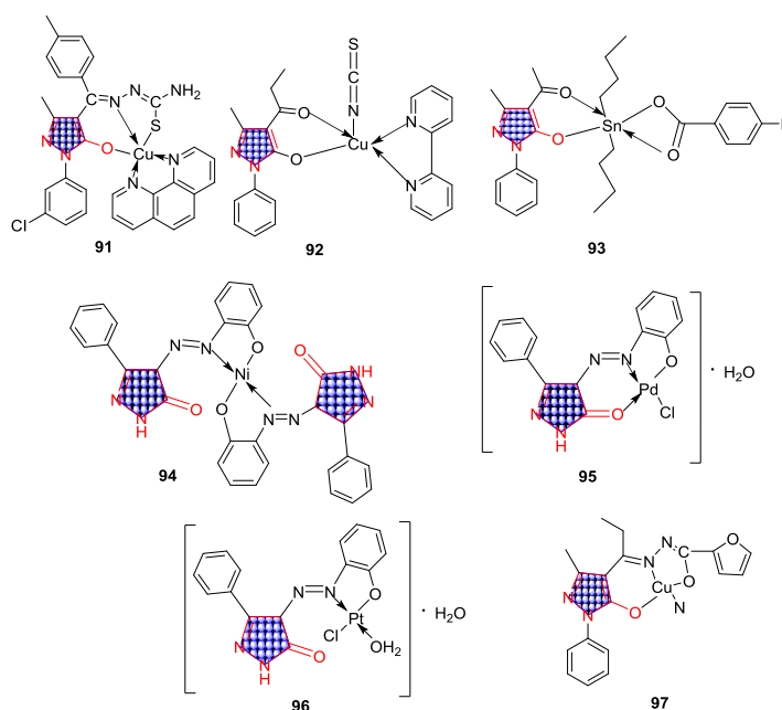
Figure 8. Coordination pyrazolone compounds as antitumor agents.
