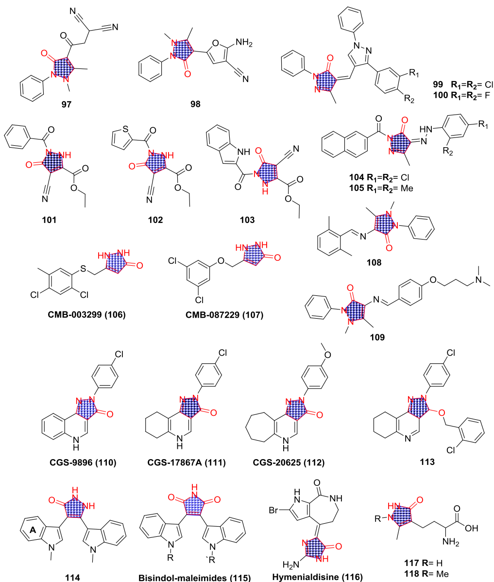
Figure 9. Pyrazolones as CNS agents.
