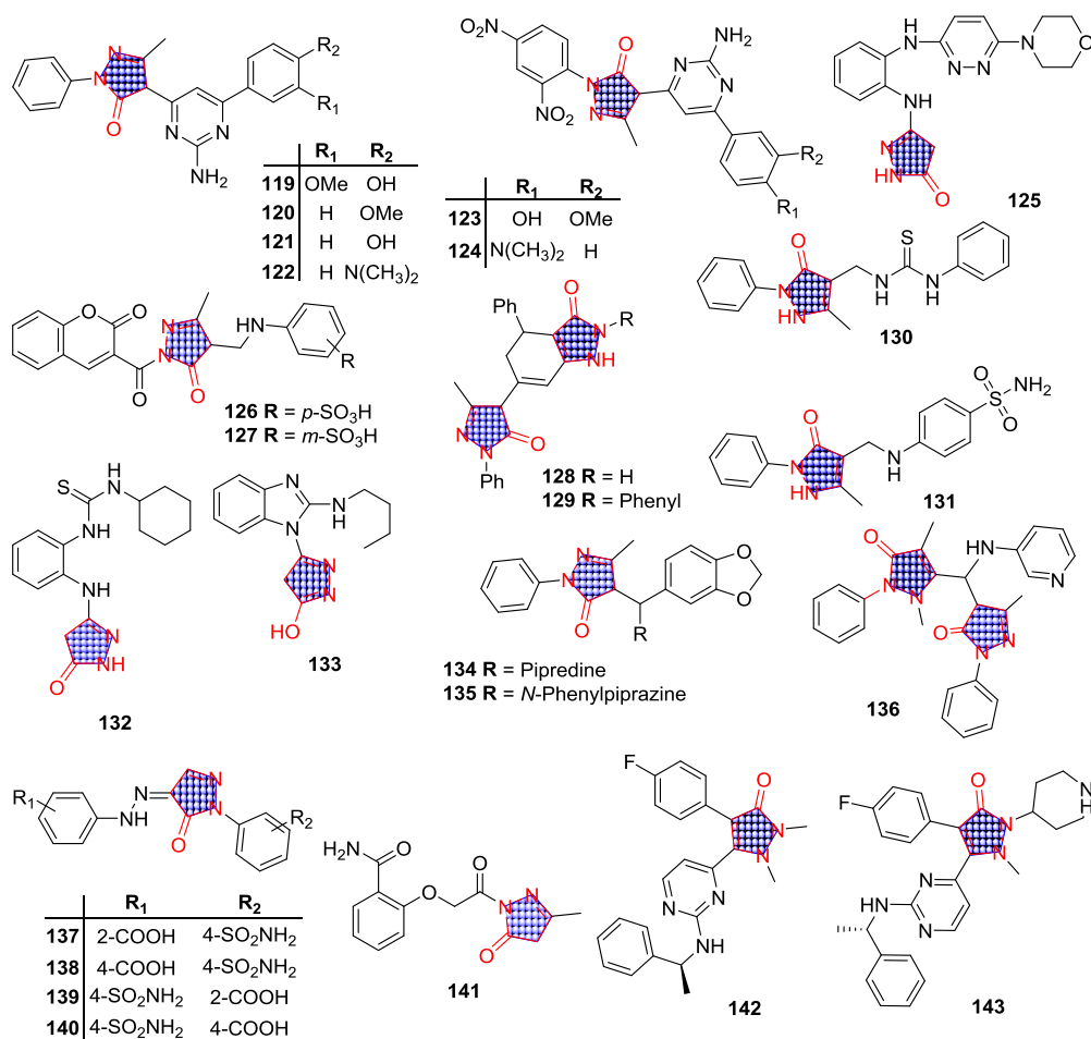
Figure 11. Pyrazolone derivatives with anti-inflammatory activity.
