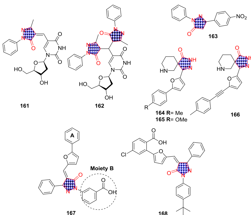
Figure 16. Antiviral of pyrazolone analogues.
