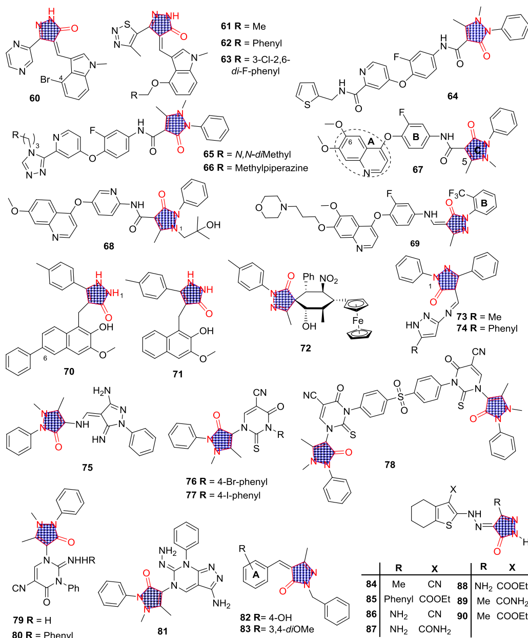
Figure 6. Pyrazolone derivatives with antitumor activity.
