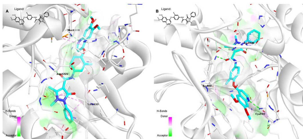
Figure 7. Resolved pharmaceutical cocrystal of pyrazolone derivative 67 with c-Met ( A , PDB ID: 3U6H) and VEGFR-2 kinase ( B , PDB ID: 3U6J).
