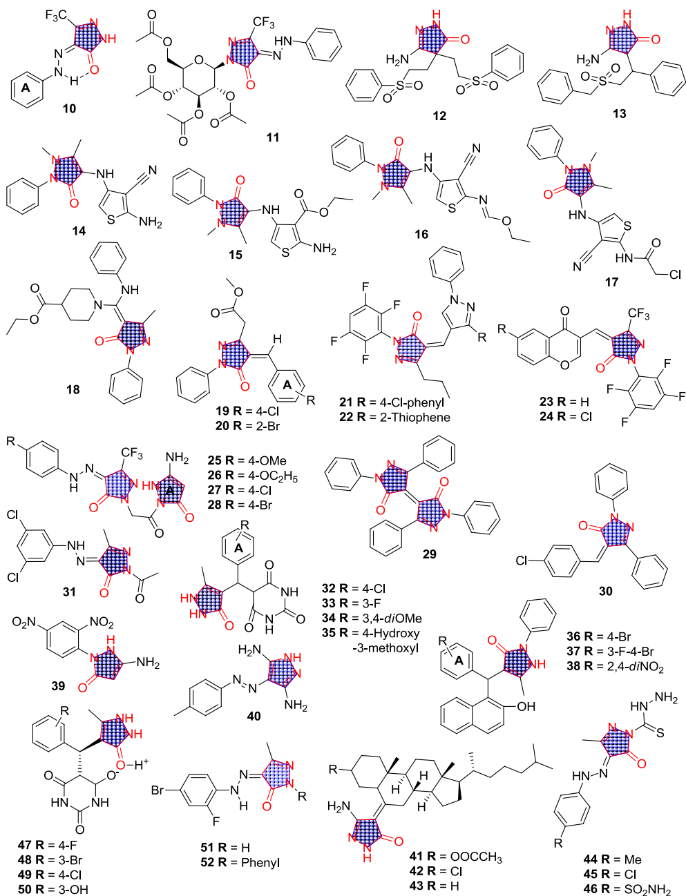
Figure 3. Pyrazolone derivatives with antimicrobial activity.
