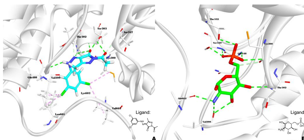
Figure 4. Ligand-protein interactions of compound 31 (A) and original ligand (B) with the active site of glucosamine-6-phosphate synthase (PDB ID: 2VF5) accomplished by Discovery Studio 2019.
