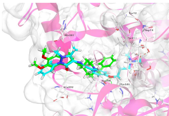
Figure 10. Ligand-protein interactions of compound 108 (blue) and donepezil (green) with AChE (PDB ID: 4EY7) accomplished by Discovery Studio 2019.
