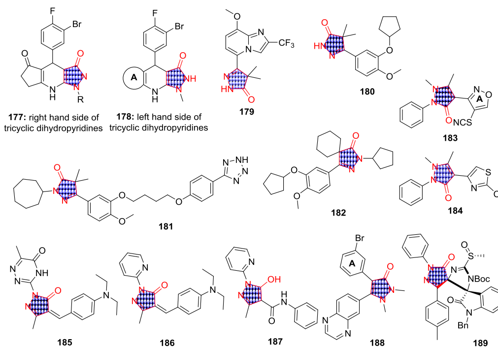
Figure 19. Pyrazolone as protein inhibitors.
