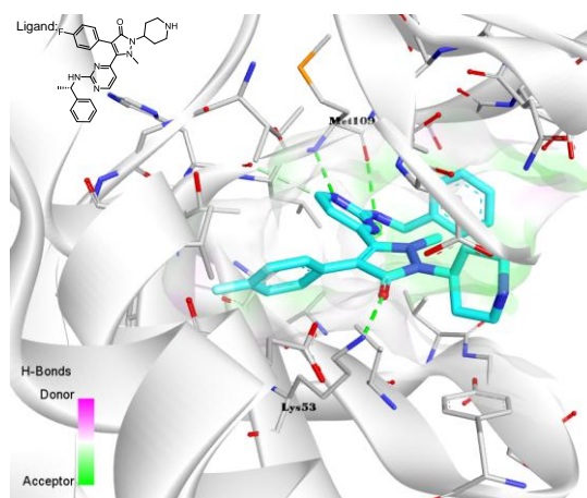
Figure 13. Resolved pharmaceutical cocrystal of pyrazolone derivative 143 with p38 kinase (PDB: 1YWR).
