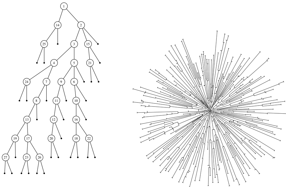
FIGURE 2. Two increasing Schröder trees
