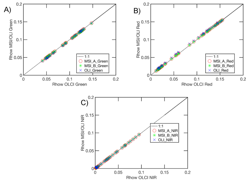
Figure 4. Using the relative spectral response of each sensor, sensor equivalent R_{how} values were derived from 50 in-situ R_{how} for OLI, MSI and OLCI. R_{how} of MSI/OLI versus OLCI in green band (A), R_{how} of MSI/OLI versus OLCI in red band (B) and R_{how} of MSI/OLI versus OLCI in NIR band (C).
