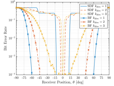
Fig. 4. Spatial BER distribution for different constellation sizes ( f_c = 2.45 GHz, B = 20 MHz, antenna spacings b = 0.5\lambda_c , SNR = 25 dB)
