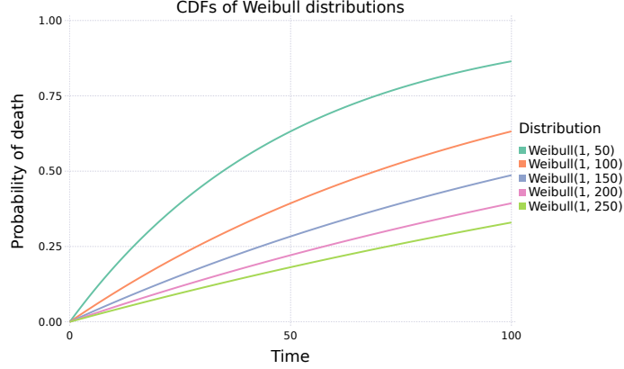
Figure 3: Examples of the functions that give the probability of death of a patient as a function of time after admission into the ICU.
