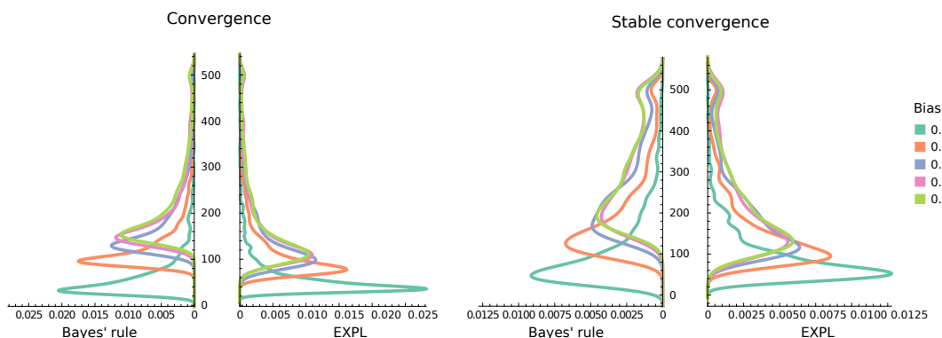
Figure 1: Paired density plots showing speed of convergence to the truth (left) and speed of stable convergence to the truth (right) for Bayes' rule and EXPL, for biases from .1 to .5. The x-axes show probability densities, the y-axes show toss numbers. Individual plots can be interpreted as showing the relative likelihood that the first time a probability above the threshold is assigned (left) / is stably assigned (right) to a hypothesis occurs at a given toss.
