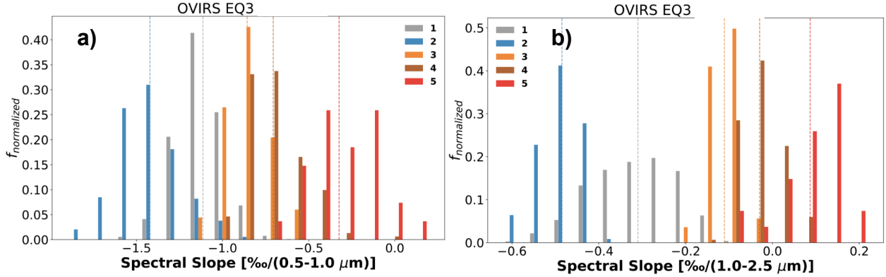
Fig. 2. Distribution of the slope of all spectra obtained for each of the five groups for q_1 = 2.0\sigma : (a) spectral slope between 0.5 and 1.0 \mu\text{m} , and (b) spectral slope between 1.0 and 2.5 \mu\text{m} . The color code is the same in both panels.
