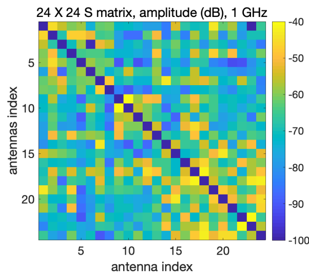
Figure 3. The 24 \times 24 scattering matrix measured in the presence of the head phantom; the self-terms are forced to zero.
