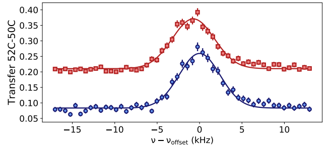
Figure 4. Test of atomic coherence. Microwave spectrum of the two-photon |50C\rangle \rightarrow |52C\rangle transition for trapped (blue circles) and untrapped (red rectangles) atoms (statistical error bars) with \nu_{\text{offset}} = 49.639071\text{ GHz} . The fraction of atoms transferred to |52C\rangle is plotted w.r.t. the detuning of the microwave source from resonance. The red points have been shifted upwards for clarity.
