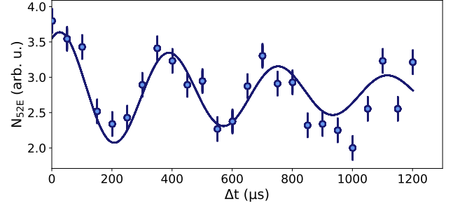
Figure 3. Trap frequency measurement. Blue circles with statistical error bars: number of atoms, N_{52E} in |52E\rangle , as a function of the time \Delta t at which the trap is switched off. Blue line: damped sinusoidal fit to the data.
