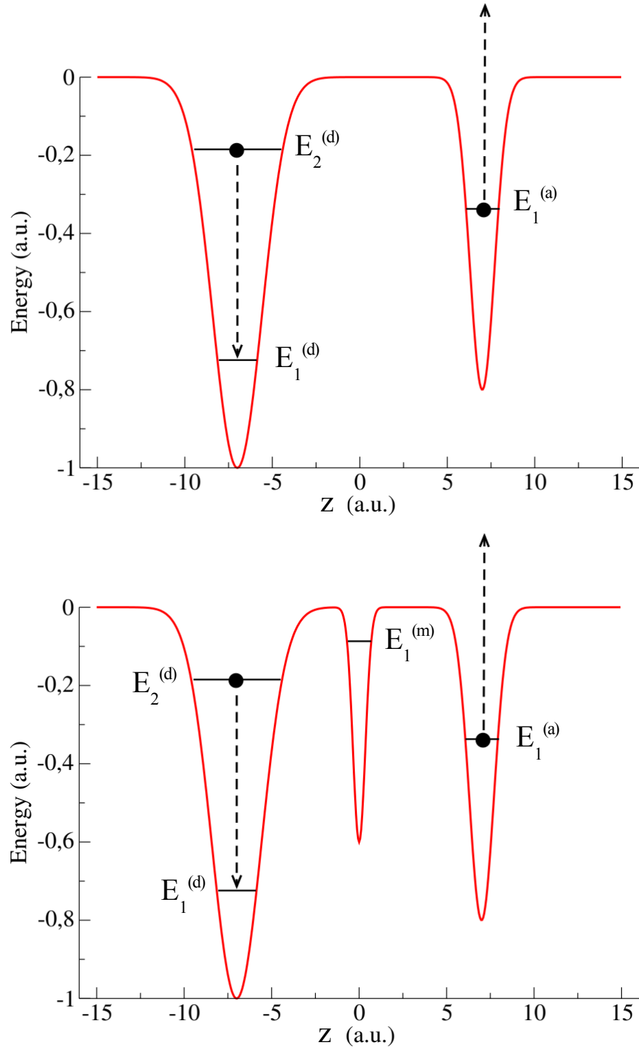
FIG. 1. Scheme of the ICD in two (upper panel) and three (lower panel) coupled quantum dots. Via ICD, the left (donor) quantum dot releases its excess energy by ionizing the right (acceptor) dot, as indicated by the arrows. The quantum dots are represented by effective one-dimensional potentials as in [10–13]. E_n^{(j)} denote the one-electron energies (see text).
