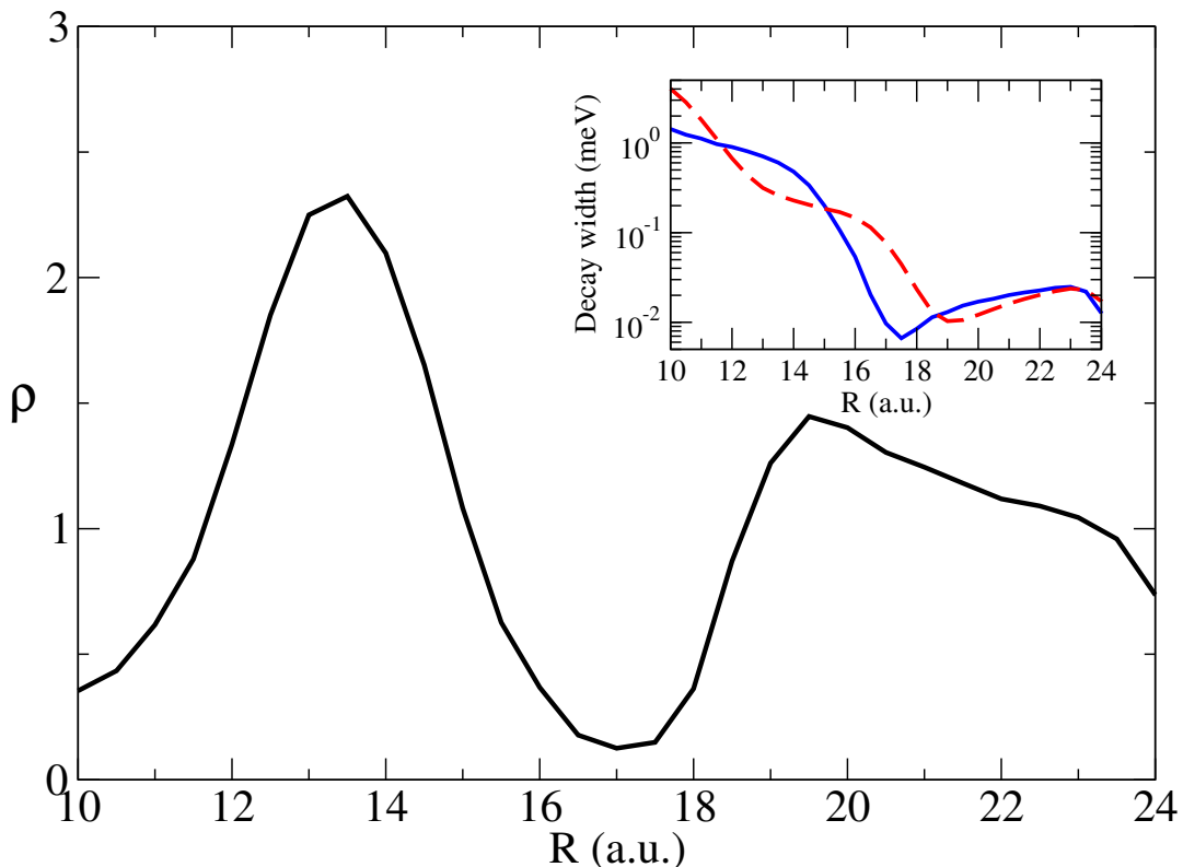
FIG. 2. Ratio between the decay widths for three and two coupled quantum dots as a function of the distance between the donor and acceptor dots ( R ). Inset: Decay widths for two (dashed red line) and three (blue line) coupled quantum dots. The parameters (see text) of the bridge quantum dot are ( Z_m=0.6 ; \sigma_m=4.0 ).
