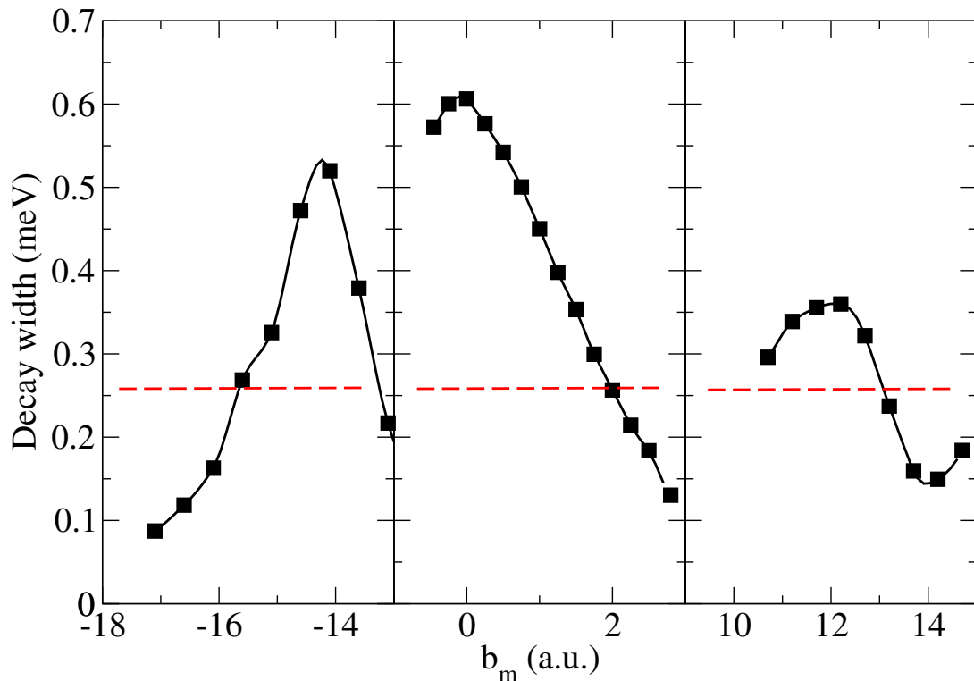
FIG. 4. Decay widths as a function of the position of the bridge quantum dot, for R = 13.5 a.u. (i.e. the donor and acceptor dots are fixed at -6.75 a.u. and 6.75 a.u., respectively.). The red dashed-line indicate the decay width in absence of the bridge. Note that we have limited the range of b_m to the values that do not change significantly the energies of the donor and acceptor dots with respect to the two coupled quantum dots case.
