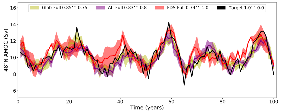
Fig. 4 Evolution of the AMOC at 48° N for global (Glob-Full, yellow), Atlantic only (Atl-Full, purple), FDS region only (FDS-Full, red). Significance of the correlations of the whole time series between each experiment and the Target are indicated on each label as ** for a 99% confidence levels
