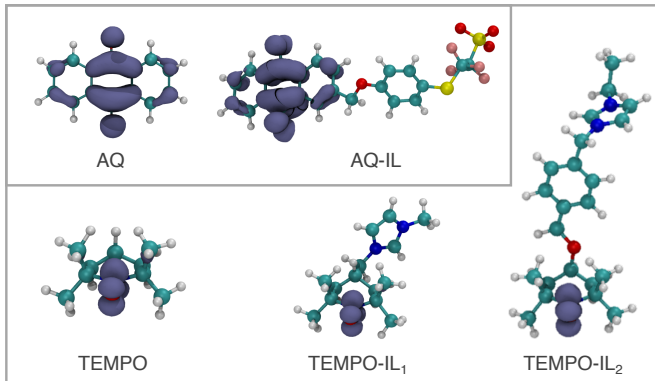
FIG. 4: Electron/hole localization from DFT for redox molecules. Top row shows the electron density (gray) for AQ^- and AQ-IL^{2-} and the bottom row shows the hole density in TEMPO^+ , TEMPO-IL_1^+ and TEMPO-IL_2^+ .
