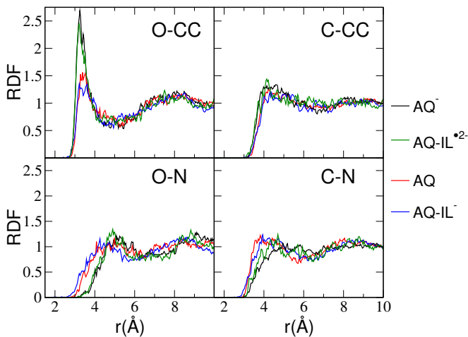
FIG. 4: Electron/hole localization from DFT for redox molecules. Top row shows the electron density (gray) for AQ^- and AQ-IL^{2-} and the bottom row shows the hole density in TEMPO^+ , TEMPO-IL_1^+ and TEMPO-IL_2^+ .
