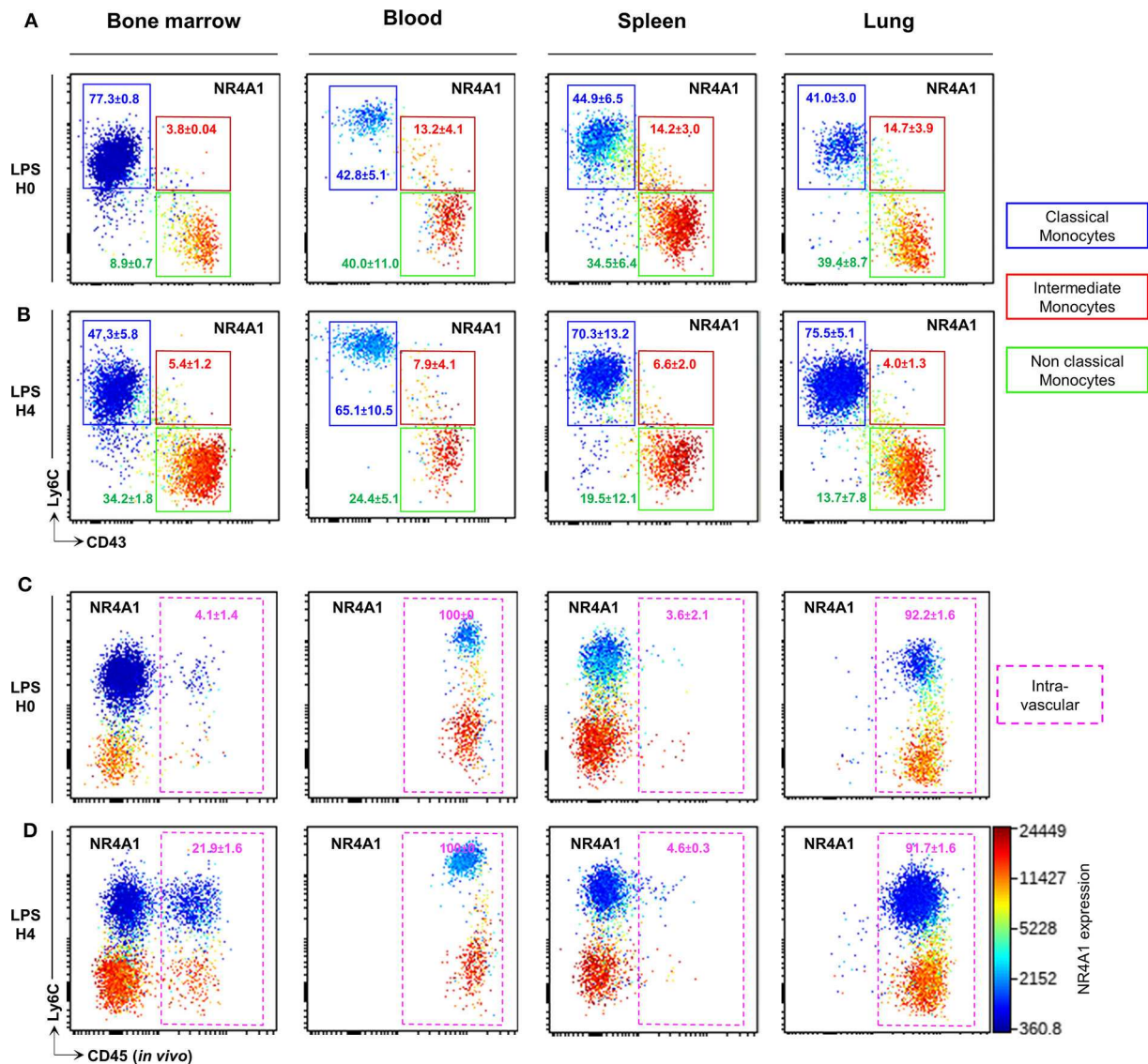
FIGURE 3 | CD43 expression identifies circulating and tissue resident NCMo subsets. Classical (blue gate), intermediate (red gate), and non-classical (green gate) monocyte subsets were gated according to Ly6C and CD43 markers expression in the bone marrow, the blood, the spleen, and the lungs before (A) and 4 h after LPS intraperitoneal injection (B). The distribution of monocyte subsets between the vasculature and the organs parenchyma was evaluated by blood tissue partitioning (intravascular CD45 staining) before (C) and 4 h after LPS intraperitoneal injection (D). Nr4a1 reporter expression (using Nr4a1 +/EGFP mouse) was presented in each dot plot in a color scale going from blue to red (A–D). Dot-plots are representative of n = 3 per group.
