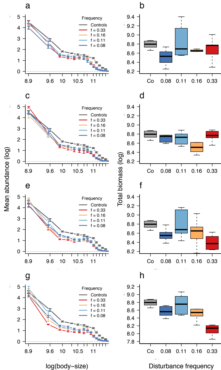
Figure S2: Effect of disturbance frequency on community size-structure and total biomass for different disturbance intensities: a-b) I = 10\% c-d) I = 30\% , e-f) I = 50\% , g-h) I = 70\% .
