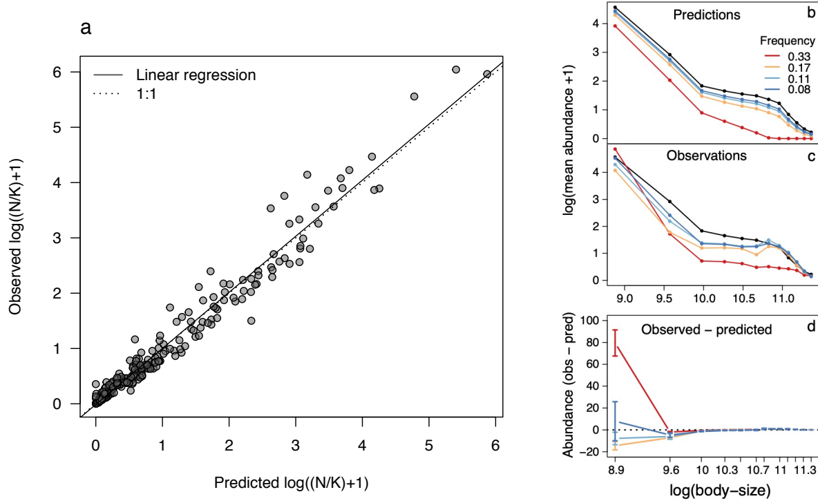
Figure 5: Comparison between experimental results and model predictions. a) Predicted vs. observed mean abundance N relative to carrying capacity K in the twelve size-classes for all the disturbance regimes ( n=240 ). Solid line: linear regression [ y = -0.012 + 1.01x , R^2 = 0.96 , p\text{-value} < 0.001 . Standard error for slope: 0.01, intercept: 0.02]. Dashed line indicates a 1:1 relationship. b) Predicted effect of disturbance frequency on the community size-structure of experimental communities. Disturbance intensity is fixed to I = 90\% ; other disturbance regimes are shown in Figs. S4-S5. Controls are in black (undisturbed environment) and axes are on a logarithmic scale. c) Observed effect of disturbance frequency on the community size-structure of experimental communities (similar to Fig. 4a). d) Difference between observed and predicted mean abundance for each size-class.
