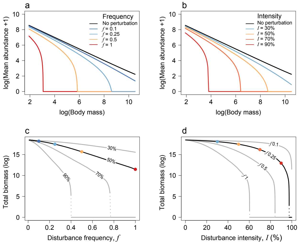
Figure 3: Effects of disturbance frequency and intensity on community size-structure and average total biomass at dynamical steady state. Analytical results derived from Equation (5). a) Effect of disturbance frequency (disturbance intensity is fixed to 50% abundance reduction), and b) disturbance intensity (disturbance frequency is fixed to 0.25) on community size-structure. c) Effect of disturbance frequency and d) intensity on average total biomass (in log), for different intensities (c) and frequencies (d), respectively. Points on the black lines in (c) and (d) show the disturbance regimes corresponding to community size-structures of the respective colors displayed in panels (a) and (b).
