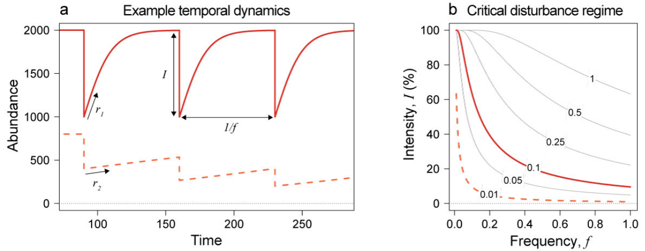
Figure 2: Population dynamics and persistence according to disturbance regime. a) Temporal dynamics of two species experiencing the same disturbance regime. Species 1 has a smaller body-size and therefore a higher growth rate than species 2. A population can persist only if its growth rate balances the long-term effect of the disturbance regime. We derive in equation (4) the mean abundance at dynamical equilibrium (i.e. temporal mean) of the persisting species experiencing varying disturbance regimes. b) Isoclines of the persistence criterion in the disturbance regime landscape according to population growth rate (numbers): on and above the line, the population of a given growth rate goes extinct. Lines with the same color code as in panel (a) correspond to the same growth rate.
