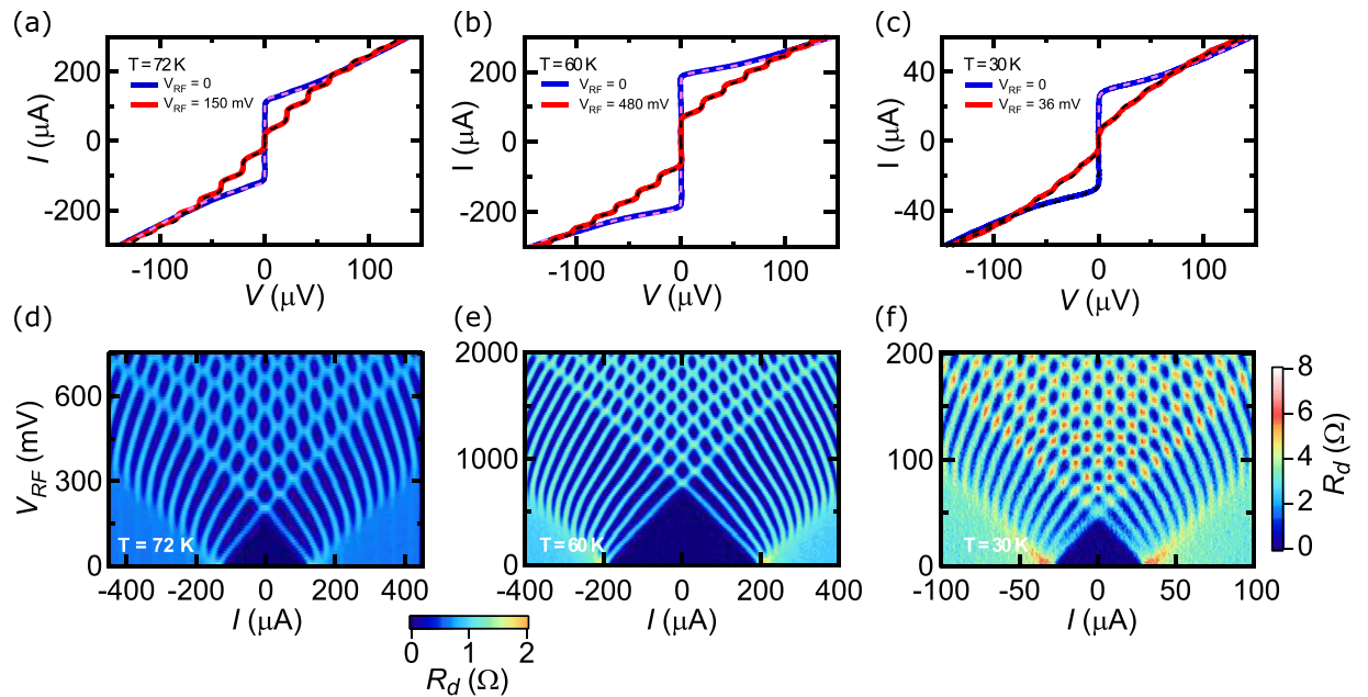
Figure 2. I - V characteristics of (a) a 200 ions/nm JJ, (b) a 400 ions/nm JJ and (c) a 600 ions/nm JJ, with (red) and without (blue) 10 GHz irradiation. Solid lines are data and dashed lines RSJ fits. Color-plot of R_d as a function of I and V_{\text{RF}} at f = 10\text{ GHz} for (d) a 200 ions/nm JJ and (e) a 400 ions/nm JJ (Color-scale at the bottom). (f) Same plot for a 600 ions/nm JJ (Color scale on the right).
