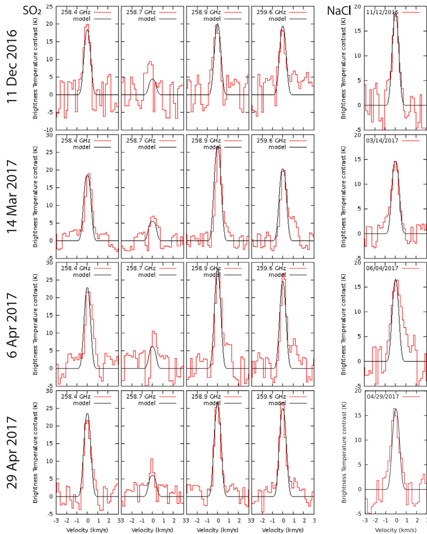
Fig. 2. Disk-averaged spectra (red) of the four SO 2 lines (left four columns) and the NaCl 260.223 GHz line (rightmost column) for the four IRAM observing tracks. The continuum was subtracted. The model results for fitting the brightness temperature (simultaneously for the four SO 2 lines) are shown in black. The corresponding images for the SO 2 258.942 GHz line and the NaCl line are shown in Fig. 1. (For interpretation of the references to color in this figure legend, the reader is referred to the web version of this article.)
