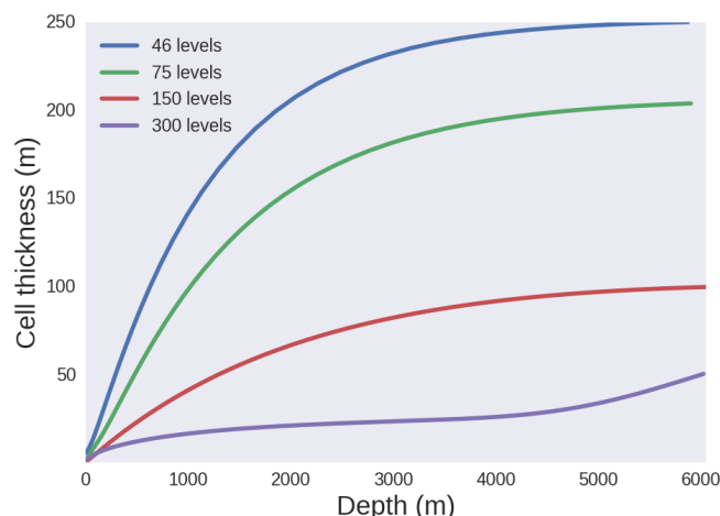
Figure A1. Grid cell thickness as a function of depth for the four vertical grids used in the study.
