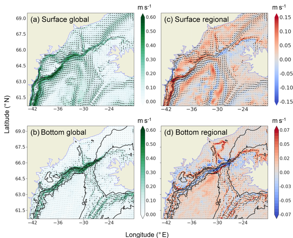
Figure 2. Surface (a) and bottom (b) mean currents (year 76) in the global ORCA12 simulation. Vectors and colours indicate current direction and speed ( \text{m s}^{-1} ). Surface (c) and bottom (d) mean currents (year 76) in the regional DSO12.L46 regional simulation. Vectors indicate the direction of the current. Colours indicate the current speed difference between the global and the regional simulation ( \text{m s}^{-1} ). Blue and red indicate that the current speed is greater or smaller in the global or regional simulation.
