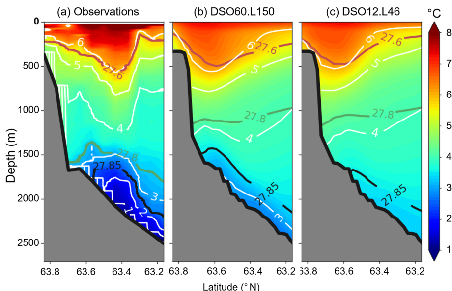
Figure 5. Potential temperature ( ^{\circ}\text{C} ) at section 29 in (a) the observations (ASOF6 section; Quadfasel, 2010), (b) the 1/60^{\circ} , 150-level simulation (annual mean), and (c) the 1/12^{\circ} , 46-level simulation (annual mean). Red, green, and black full lines are isopycnals 27.6, 27.8, and 27.85. White lines are isotherms in 1^{\circ}\text{C} intervals. In panel (b), section 29 is outside (100 km downstream) the 1/60^{\circ} AGRIF zoom, so the effective resolution is 1/12^{\circ} , but the water masses acquired their properties upstream within the 1/60^{\circ} resolution zoom.
