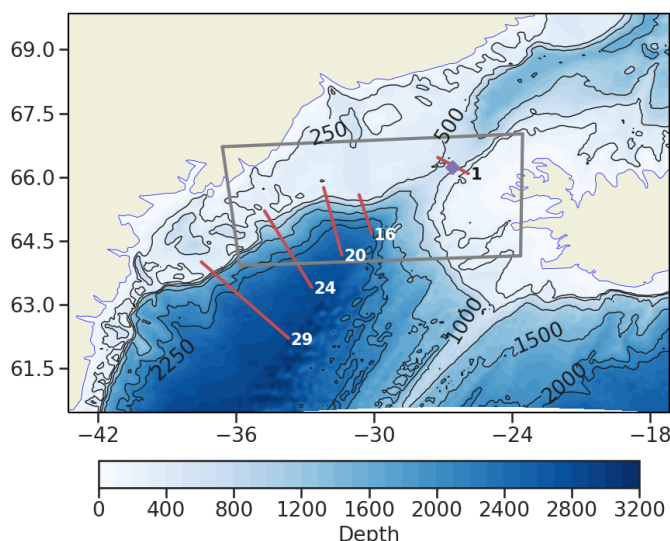
Figure 1. Regional model domain with the ocean depth in colour. The 250, 500, 1000, 1500, and 2000 m depth isobaths are contoured in black. The grey box indicates the region where the two-way grid refinement ( 1/36 and 1/60^\circ ) is applied in some simulations. The locations of the various sections used to monitor the model solution are shown by the red lines. Section 1 is the reference section chosen for the sill.
