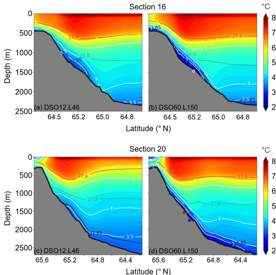
Figure 6. Distribution with depth of the annual mean temperature (fifth year of model run) at section 16 (Dohrn Bank array) for (a) simulation DSO12.L46 and (b) simulation DSO60.L150 (in the refined grid), as well as at section 20 (Spill Jet section) for (c) simulation DSO12.L46 and (d) simulation DSO60.L150 (in the refined grid). Temperature ( ^{\circ}\text{C} ) is represented by colours with white contours. Potential density values ( \sigma_0 ) are shown by the contour lines coloured in red (27.6), green (27.8), and black (27.85). The white-rimmed dot in (b) corresponds to the location of the profiles displayed in Fig. 15, and the red-rimmed and blue-rimmed dots in (d) correspond to the locations of the profiles displayed in Fig. 13.
