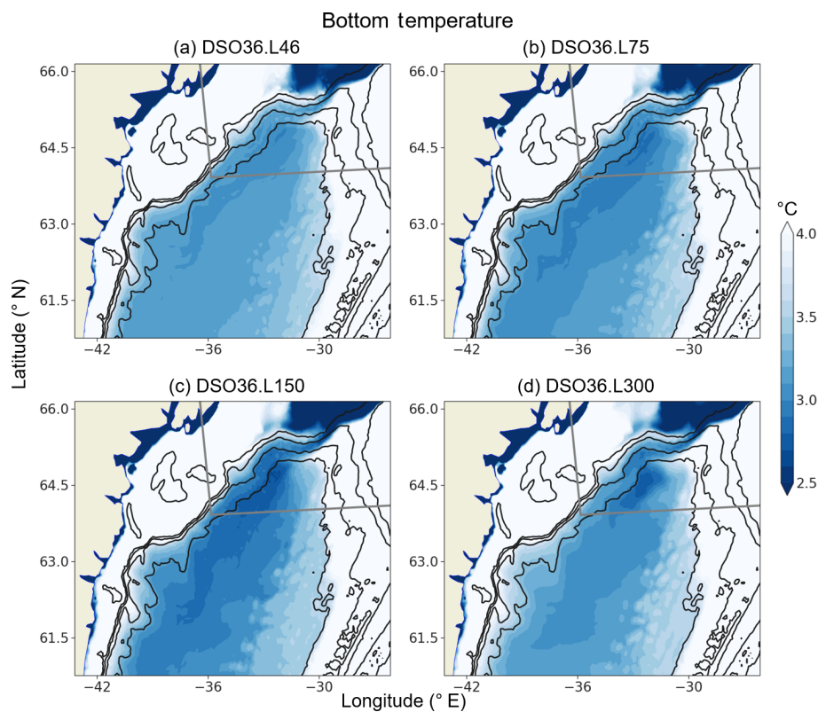
Figure 11. Annual mean of the bottom temperature of year 5 of simulations using grid refinement ( 1/36^{\circ} ): (a) DSO36.L46, (b) DSO36.L75, (c) DSO36.L150, (d) DSO36.L300. Isobaths 500, 1000, 1500, and 2000 m are contoured in black.
