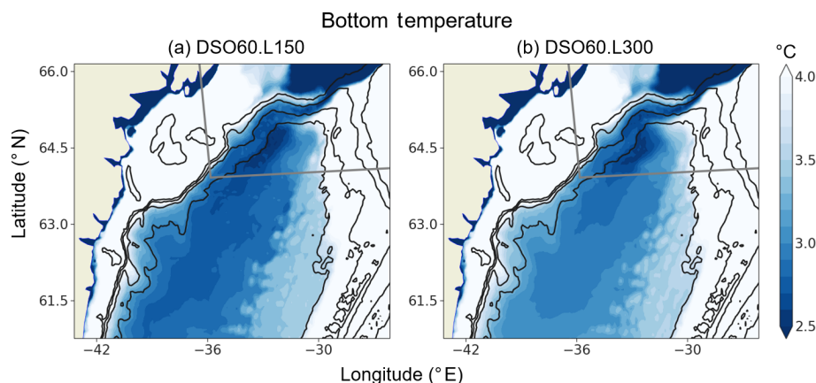
Figure 12. Annual mean of the bottom temperature in the fifth year of simulations using a grid refinement of 1/60^\circ for (a) 150 vertical levels (DSO60.L150) and (b) 300 vertical levels (DSO60.L300). Isobaths 500, 1000, 1500, and 2000 m are contoured in black. The grey box indicates the area of refinement.
