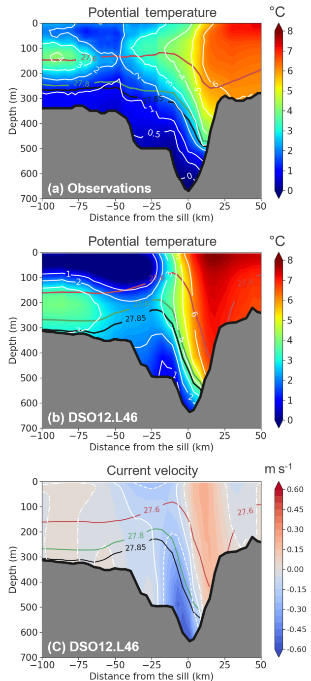
Figure 4. Mean flow characteristics (annual mean of year 76) in the global simulation for a section across the sill. Temperature (°C) is represented by colours and white contours for (a) the observations (Mastropole et al., 2017) and (b) the control simulation (DSO12L46 1/12° and 46 vertical levels). Potential density values ( \sigma_0 ) are shown by the contour lines coloured in red (27.6), green (27.8), and black (27.85). (c) The velocity normal to the section in the control simulation (with southward velocity in blue being negative). White lines indicate the 0 \text{ m s}^{-1} contour (dashed-dotted line), the -0.1 \text{ m s}^{-1} contour (full line), and the -0.2 \text{ m s}^{-1} contour (dashed line).
