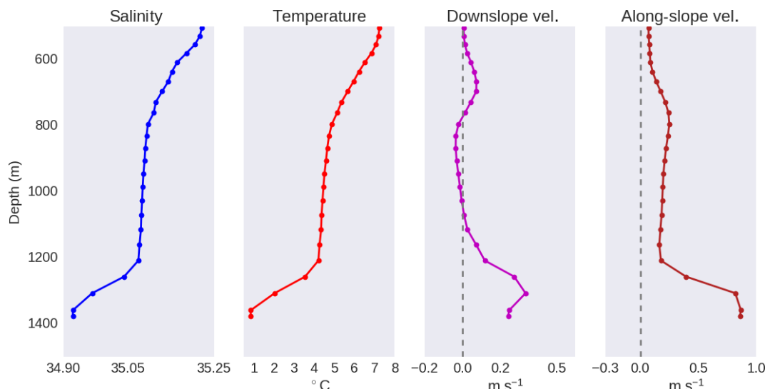
Figure 15. Vertical profiles of the physical properties of the overflow plume in simulation DSO60.L150 (hour 10 on 1 February of year 5) at section 16 for the location indicated with a white-rimmed dot in Fig. 6b. (a) Salinity, (b) temperature, (c) cross-slope velocity, and (d) along-slope velocity.
