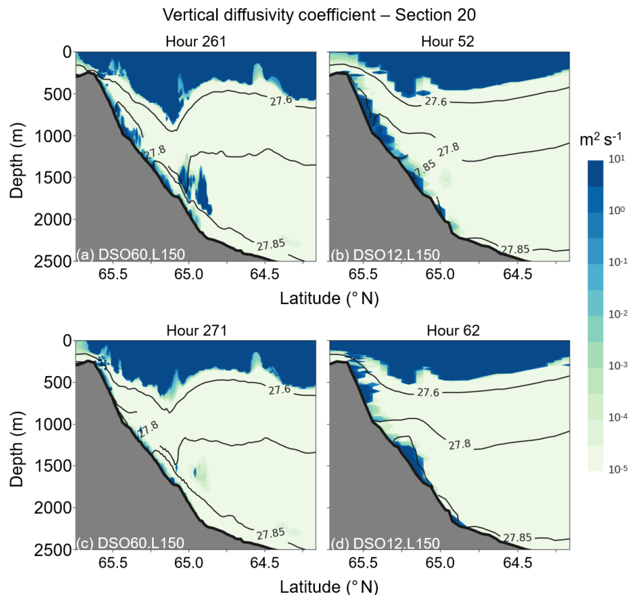
Figure 14. Vertical diffusivity coefficient ( K_z , hourly mean) at section 20 in simulations (a, c) DSO60.L150 (in the refined grid) and (b, d) DSO12.L150 in wintertime (with a 10 h difference). In black: contours of isopycnals 27.6, 27.80, and 27.85.
