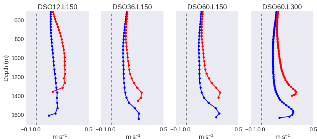
Figure 13. Vertical profiles (annual mean) of the quasi-along-slope velocity (i.e. velocity normal to the section) at the two locations of section 20 indicated in Fig. 6d for simulations (a) DSO12.L150, (b) DSO36.L150, (c) DSO60.L150, and (d) DSO60.L300.
