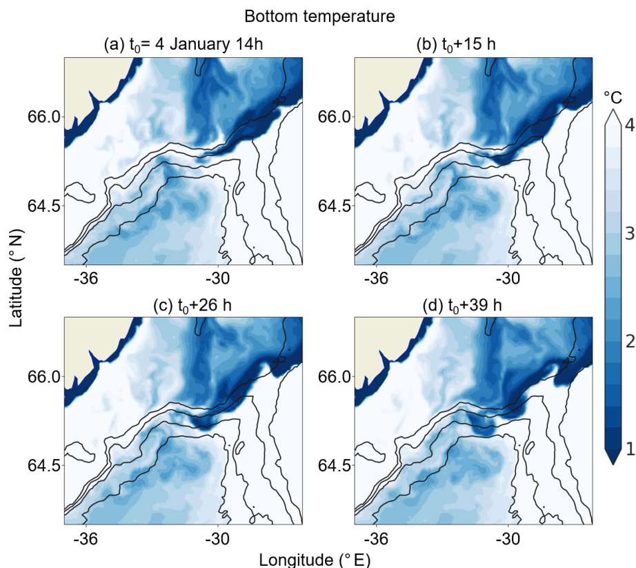
Figure 16. Hourly snapshots of bottom temperature in simulation DSO60.L150 for (a) 4 January at time t_0 = 14 h, (b) time t = t_0 + 15 h, (c) time t = t_0 + 26 h, and (d) time t = t_0 + 39 h. The 500, 1000, 1500, and 2000 m isobaths are contoured.
