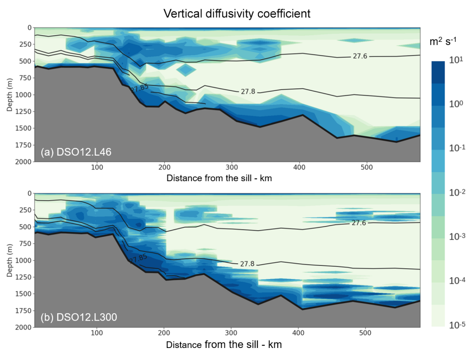
Figure 9. Vertical diffusivity coefficient ( K_z , summer mean in the fifth year of simulation) along the path of the vein calculated for (a) simulation DSO12.L46 and (b) simulation DSO12.L300. Potential density values ( \sigma_0 ) are shown by the contour lines.
