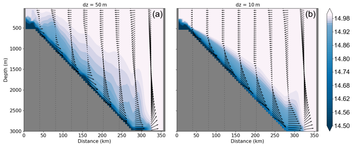
Figure 10. Idealized experiment simulating the rationale explored in Fig. 7 of Winton et al. (1998). Cold water ( 10^{\circ}\text{C} ) descends a shelf break in a configuration with ambient water at 15^{\circ}\text{C} after 9 d of simulation. Two vertical resolutions are used: (a) \Delta z = 50 m, (b) \Delta z = 10 m. Temperature ( ^{\circ}\text{C} ) is represented by colours. Vectors represent the velocity, with the vertical velocity being re-scaled according to the grid aspect ratio in the case in panel (a).
