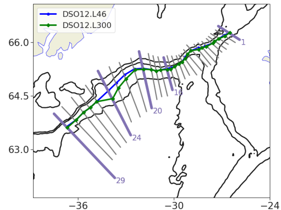
Figure B1. Overflow path. Contours show the 500, 1000, and 2000 m depth isobaths. The locations of the various sections used to monitor the model solution are indicated by grey and purple lines. The blue and green dots indicate for each section the location of the centre of the vein of the DSO in the control simulation (blue, DSO12.L46) and in the 1/12^\circ 300-level simulation (green, DSO12.L300); the blue and green lines show the path of the overflow in these simulations.
