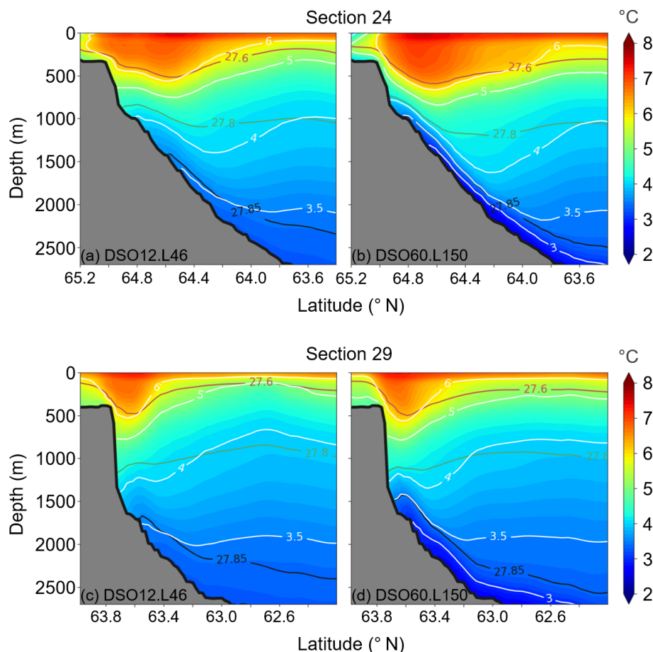
Figure 7. As in Fig. 6 at section 24 (TTO array) for (a) simulation DSO12.L46 and (b) simulation DSO60.L150, as well as at section 29 (Angmagssalik array) for (c) simulation DSO12.L46 and (d) simulation DSO60.L150.
