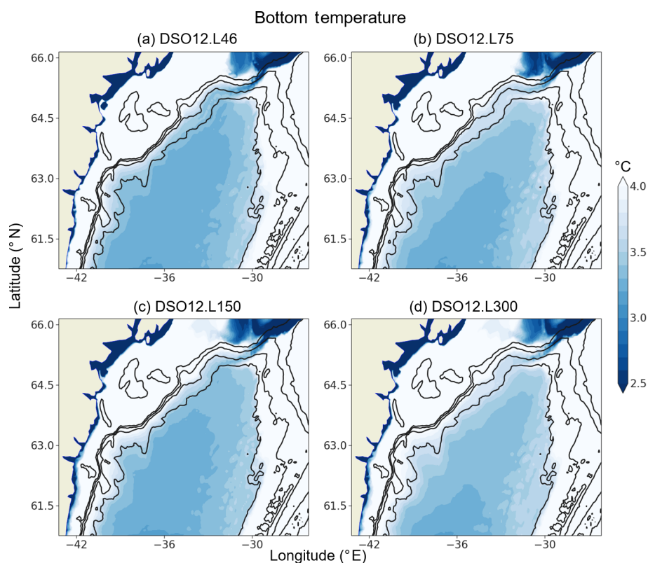
Figure 8. Annual mean bottom temperature (fifth year of simulation; °C) at 1/12^\circ horizontal resolution in simulations with differing numbers of vertical levels: (a) 46 levels (DSO12.L46), (b) 75 levels (DSO12.L75), (c) 150 levels (DSO12.L150), and (d) 300 levels (DSO12.L300). Isobaths 500, 1000, 1500, and 2000 m are contoured in black.
