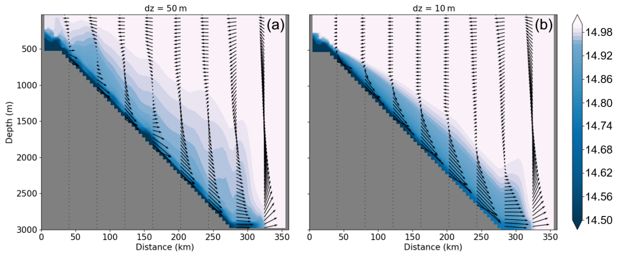
Figure 10. Idealized experiment simulating the rationale explored in Fig. 7 of Winton et al. (1998). Cold water ( 10\text{ }^{\circ}\text{C} ) descends a shelf break in a configuration with ambient water at 15\text{ }^{\circ}\text{C} after 9 d of simulation. Two vertical resolutions are used: (a) \Delta z = 50\text{ m} , (b) \Delta z = 10\text{ m} . Temperature ( ^{\circ}\text{C} ) is represented by colours. Vectors represent the velocity, with the vertical velocity being re-scaled according to the grid aspect ratio in the case in panel (a).
