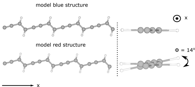
FIG. 4: Model PDA structures, constructed by substituting the side-chains of the real materials of Figure 3 with hydrogen atoms. While the two model systems might look identical when viewed from the side (left), viewing them in the direction in which the chains lie (right) emphasizes that the blue structure is planar, while a finite torsion occurs between subsequent monomers of the red structure.
