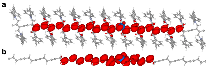
FIG. 6: Exciton wavefunction of a the real red PDA chains and b the model red chains. The electron density is visualized in red for a hole fixed at the position indicated by a blue sphere.
