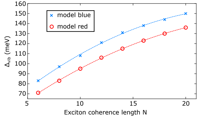
FIG. 12: The dependence of the width \Delta_{\text{vib}} of the two model PDA chains, on the exciton coherence length.
