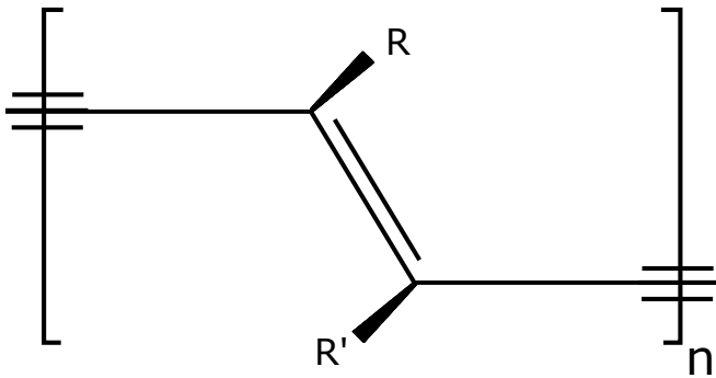
FIG. 2: The structure of a diacetylene monomer, which generally coincides with the unit cell of an infinite and periodic crystal of polydiacetylene.
