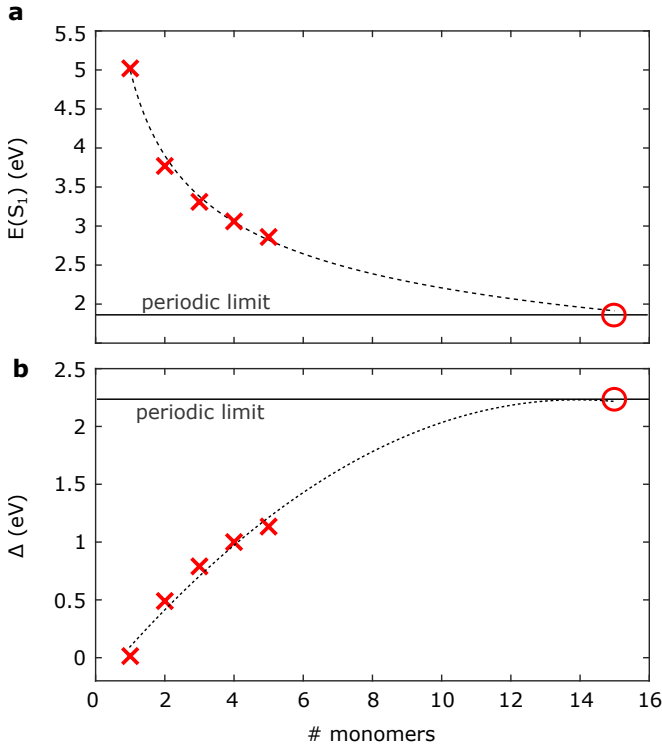
FIG. 10: The exciton energy (panel a ) and stop-band width (panel b ) for chains consisting of a different number of diacetylene monomers N . Since the constructed oligomers are planar, the periodic limit of the model blue chains is approached for a larger number of monomers.
