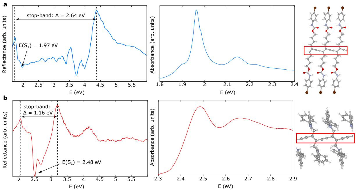
FIG. 3: Experimental reflection and absorption spectra of two studied variants of polydiacetylene: a blue chains and b red chains. The stop-band width of the two structures is approximately determined from the reflectivity spectra. The polymer structures are given alongside the experimental plots, with the polymer backbone highlighted in red rectangles, in order to distinguish it from the side-chains. Carbon atoms are denoted in light gray, hydrogen in white, oxygen in red, nitrogen in light blue and bromine in brown.
