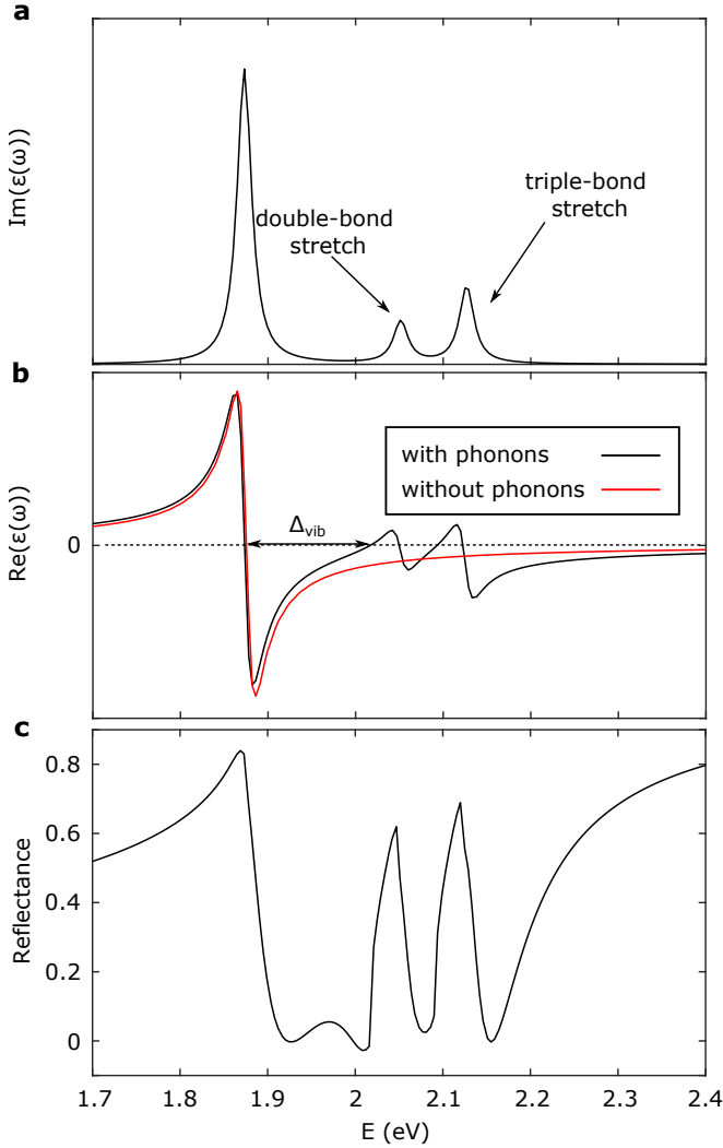
FIG. 11: The imaginary (panel a ) and real part (panel b ) of the dielectric response of the model blue chains, once the effect of phonons is accounted for. The main extra contributions to the structure of \epsilon(\omega) , compared to the disorder-free case, arise due to the effect of the carbon-carbon double- and triple-bond stretch. Comparing the structure of \text{Re}(\epsilon(\omega)) for the cases with and without phonons, we find that dynamic disorder leads to ‘breaks’ within the region of \text{Re}(\epsilon(\omega)) < 0 . This leads to a richer structure for the reflectance in panel c , compared to the disorder-free case of Figure 7.
