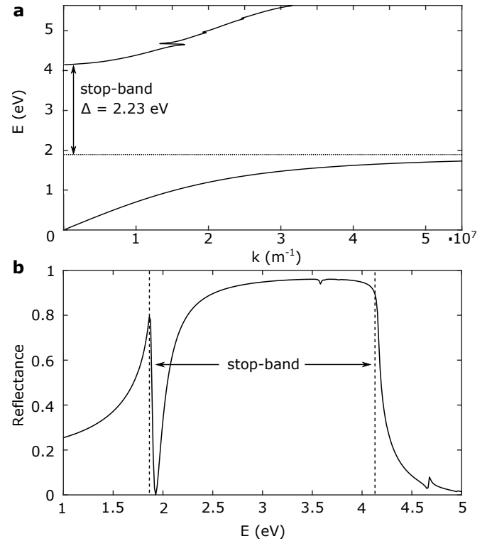
FIG. 7: Calculated a polariton dispersion and b reflectance of the model blue PDA chains, highlighting the stop-band of width \Delta = 2.23 eV.
