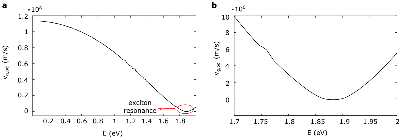
FIG. 8: Polariton group velocity in model blue chains, for different energies of the incident light. Panel a shows a large region of frequencies, whereas panel b provides a closer view of the region close to the resonance with the exciton.
