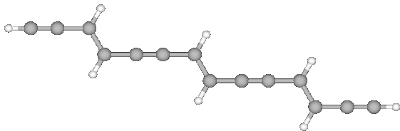
FIG. 9: A hydrogen-terminated trimer of diacetylene.
