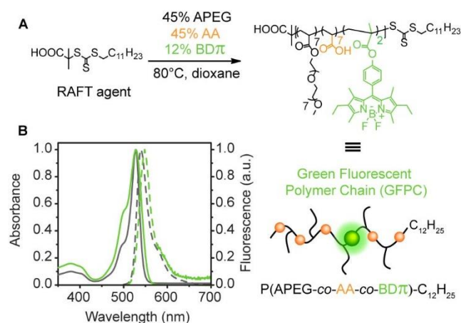
Figure 1. A: synthesis of GFPC via RAFT polymerization; B: absorption (full lines) and fluorescence emission (dotted lines, \lambda_{exc} = 495nm) normalized spectra of BD \pi monomer (black) in toluene and GFPC (green) in water (pH = 7.0).
