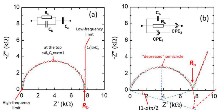
Figure 3. (a) Nyquist impedance plot of an idealized fast-ionic conductor (FIC). The semicircle centered at R_b/2 represents the response of the R_b, C_b parallel element and straight line is the capacity of the electrolyte/electrode interface of impedance 1/j\omega C_e . (b) Nyquist impedance plot of a FIC sample. The depressed semicircle reflects the combination of R_b, C_b, CPE_1 and the inclined straight line represents the double-layer capacity of the inhomogeneous electrode surfaces.
