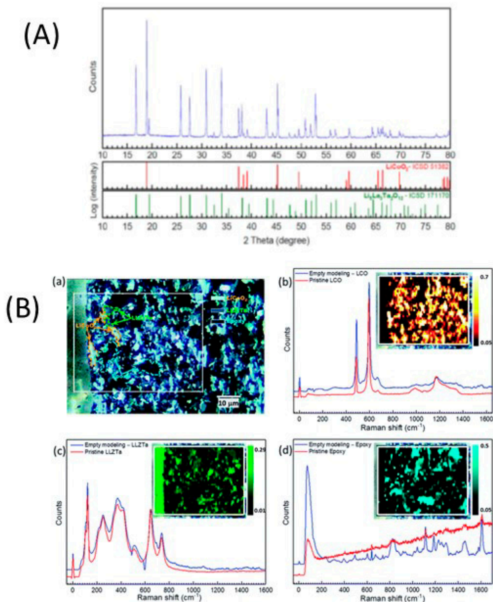
Figure 25. (A) X-ray diffraction patterns of \text{LiCoO}_2/\text{Li}_{6.6}\text{La}_3\text{Zr}_{1.6}\text{Ta}_{0.4}\text{O}_{12} composite cathode with the mass ratio of 1:1 that was sintered at 1050\text{ }^\circ\text{C} for 30 min in air. (B) High-resolution micro-Raman mapping of the cross-section of the ASSLB. (a) Optical image of the ASSLB cross-section and its mapping area. Raman mappings and spectra of (b) \text{LiCoO}_2 , (c) Ta-LLZO, and (d) epoxy. Reproduced with permission from [13]. Copyright 2019 Royal Society of Chemistry.
