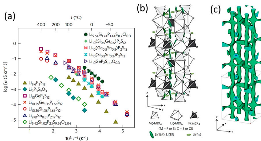
Figure 20. (a) Arrhenius conductivity plots of \text{Li}_{11-x}\text{M}_{2-x}\text{P}_{1+x}\text{S}_{12} ( M = \text{Ge}, \text{Sn}, \text{Si} ) structures, \text{Li}_{9.6}\text{P}_3\text{S}_{12} , and \text{Li}_{9.54}\text{Si}_{1.74}\text{P}_{1.44}\text{S}_{11.7}\text{Cl}_{0.3} electrolytes. (b) Crystal structure of \text{Li}_{9.54}\text{Si}_{1.74}\text{P}_{1.44}\text{S}_{11.7}\text{Cl}_{0.3} . The thermal ellipsoids were drawn with 50% probability. The framework structure consists of one-dimensional polyhedral chains (edge-sharing M(4d)X_4 and \text{Li}(4d)X_6 ) connected by \text{P}(2b)X_4 tetrahedra. Conducting Li is located at the interstitial \text{Li}(16h) , \text{Li}(8f) and \text{Li}(4c) sites. (c) Nuclear distributions of Li atoms in \text{Li}_{9.54}\text{Si}_{1.74}\text{P}_{1.44}\text{S}_{11.7}\text{Cl}_{0.3} at 25^\circ\text{C} calculated using the maximum entropy method at the iso-surface level of -0.06 \text{ fm } \text{\AA}^{-3} . Reproduced with permission from [296]. Copyright 2016 Springer.
