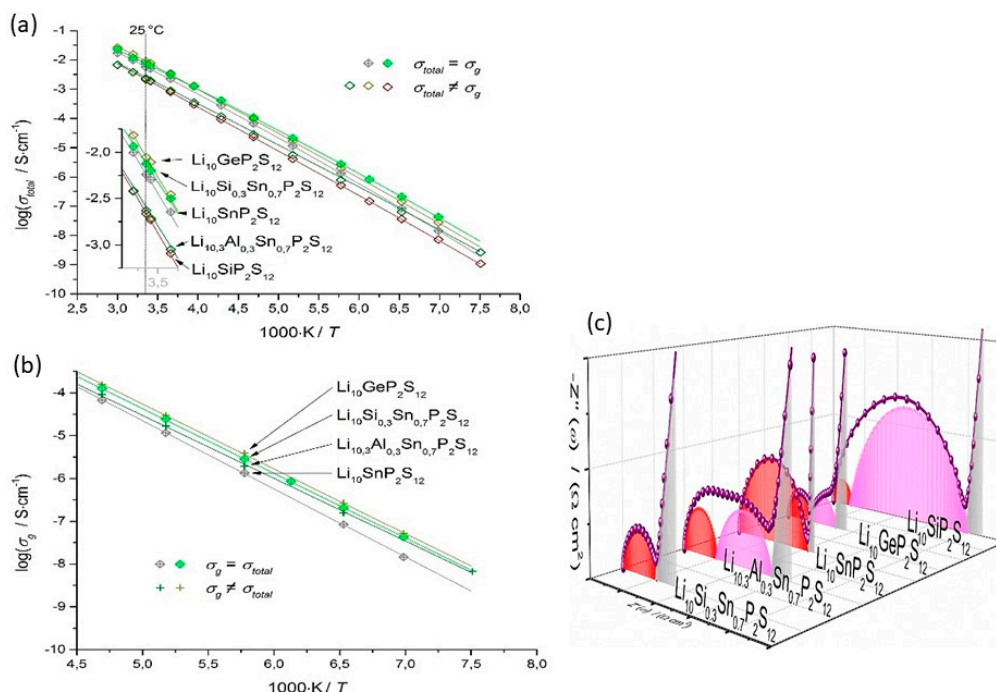
Figure 19. (a) Arrhenius plot of the total conductivities and quadratic best fit curves. The magnified image illustrates the temperature range of 0\text{--}40 \text{ }^\circ\text{C} . (b) Arrhenius plot of the grain conductivities and corresponding linear best fits in the temperature range of -140 to -60 \text{ }^\circ\text{C} . (c) Nyquist plots of electrolyte compositions. Reproduced with permission from [292]. Copyright 2016 Elsevier.
