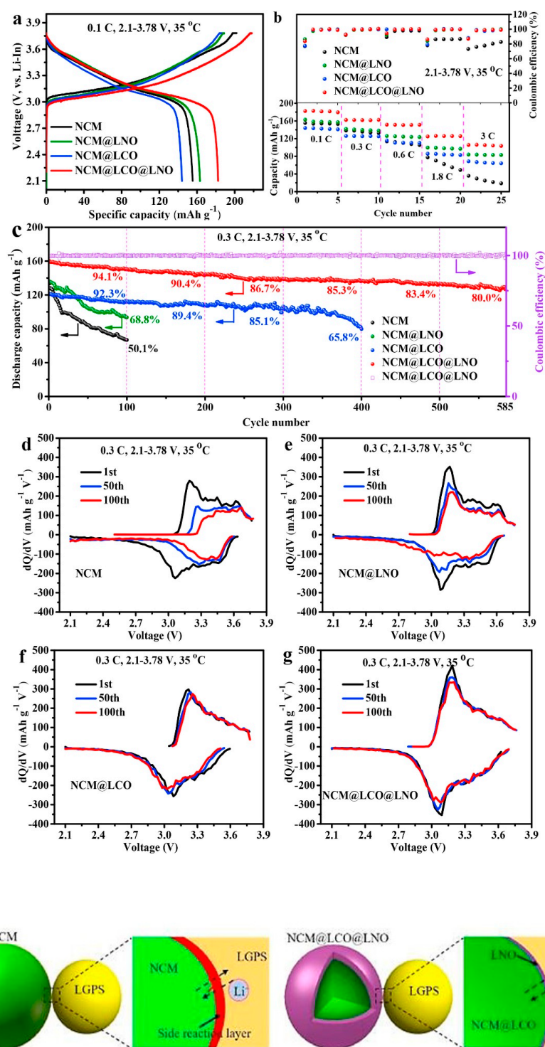
Figure 21. Electrochemical performances of NMC-811, NMC@LNO, NMC@LCO, and NMC@LCO@LNO cathodes for all-solid-state Li-ion batteries (ASSLB) with \text{Li}_{9.54}\text{Si}_{1.74}\text{P}_{1.44}\text{S}_{11.7}\text{Cl}_{0.3} as the solid electrolyte at 35 °C. Here NMC811, LCO, and LNO denote \text{LiNi}_{0.8}\text{Co}_{0.1}\text{Mn}_{0.1}\text{O}_2 , \text{Li}[(\text{Ni}_{0.8}\text{Co}_{0.1}\text{Mn}_{0.1})_{0.9}\text{Co}_{0.1}]\text{O}_2 , and \text{LiNbO}_3 , respectively. (a) Initial charge–discharge, (b) rate performance, and (c) cycle performance curves after the rate performance test ( 1\text{C} = 200\text{ mA g}^{-1} ). (d)–(g) dQ/dV curves of the four ASSLB cathodes at the 1st, 50th, and 100th cycle at 35 °C. (h) Schematic diagrams of the mitigation of the side reaction by NBO coating. Reproduced with permission from [298]. Copyright 2020 Elsevier.
