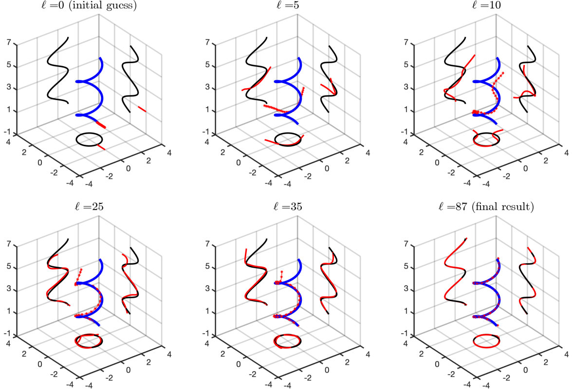
Figure 6.6: Reconstruction of the helical scatterer from Example 6.3. The top-left plot shows the initial guess, and the bottom-right plot shows the final reconstruction.
