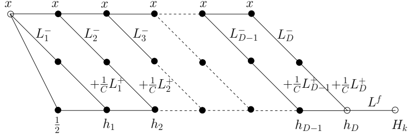
FIGURE 3.2. Structure of the Neural Network associated to the formula (3.7) and to the iterations (3.8). The top line reproduces x , it is called a source channel. The bottom line is the collation channel which realizes the addition in (3.8), it is called a collation channel. The intermediate lines correspond to the calculation of the different affine functions. The black bullets are the Neurons, they represent the application of the ReLU function with threshold T . The Neurons leave unchanged terms in the source channel and in the collation channel. The three empty bullets at the input and at the output signal that no ReLU is applied.
