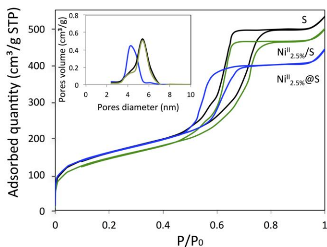
Figure S2: N_2 adsorption-desorption isotherms at -196^\circ\text{C} and pores size distributions of the calcined samples: S (black), \text{Ni}^{\text{II}}_{2.5\%}/S (green) and \text{Ni}^{\text{II}}_{2.5\%}@S (blue, prepared using the one-pot strategy).
