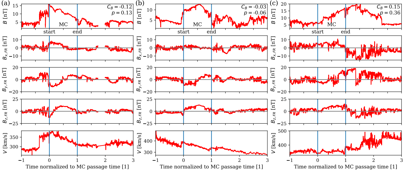
Fig. 1. Example of three MC profiles illustrating the variety of the observed asymmetric profiles of B(t) for a comparable velocity magnitude. (a) 1 November 2012, (b) 4 March 1998, and (c) 3 September 2002. From top to bottom, the panels show the magnetic field magnitude ( B ), its components ( B_{x,FR} , B_{y,FR} , B_{z,FR} ) in the FR frame (Fig. A.1), and the plasma velocity V . The time axis is normalised with the MC boundaries: t_{start} = 0 and t_{end} = 1 .
