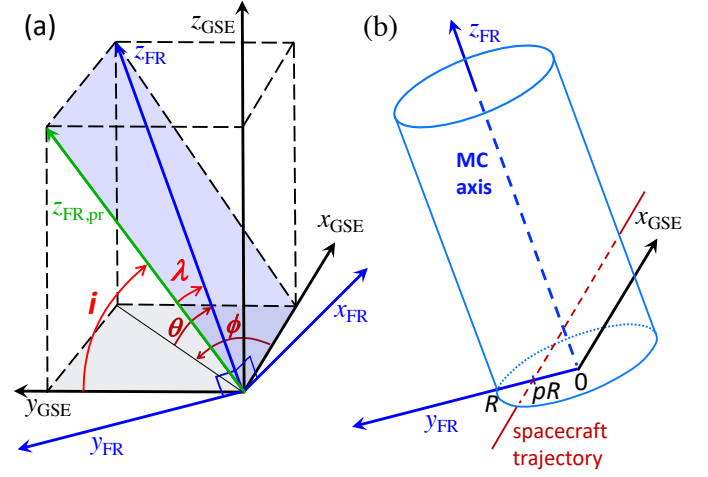
Fig. A.1. Definitions of the GSE and FR coordinate systems, the angles defining the FR axis orientation ( \theta, \phi ), or ( \lambda, i ), and the impact parameter p . In the FR frame, the rectilinear spacecraft trajectory cut y_{\text{FR}} axis at the pR value (with R the FR radius).
