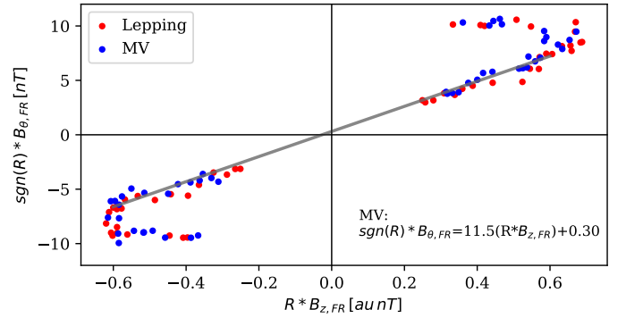
Fig. 9. Scatter plot of sgn(R) B_{\theta,FR} as a function of R B_{z,FR} using the median profiles of the SEA of Fig. 6. The variable R is considered negative in the inbound and positive in the outbound in order to separate the two regions. The grey line corresponds to the linear least square fit for the MV (blue points) in the range -0.06 au < R < 0.06 au . The y-intercept ( y_0 = 0.3 ) can be approximated to zero, so that the slope of the linear fit approximates to the twist.
