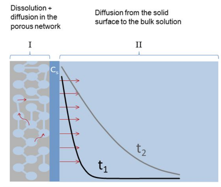
Figure 3: Scheme of the dissolution process of a mesoporous silica film with (red arrows) dissolved silicate species diffusion pathways, and black and gray curve are silicate diffusion layer concentration profiles represented at two different dissolution times t_1 and t_2 .
