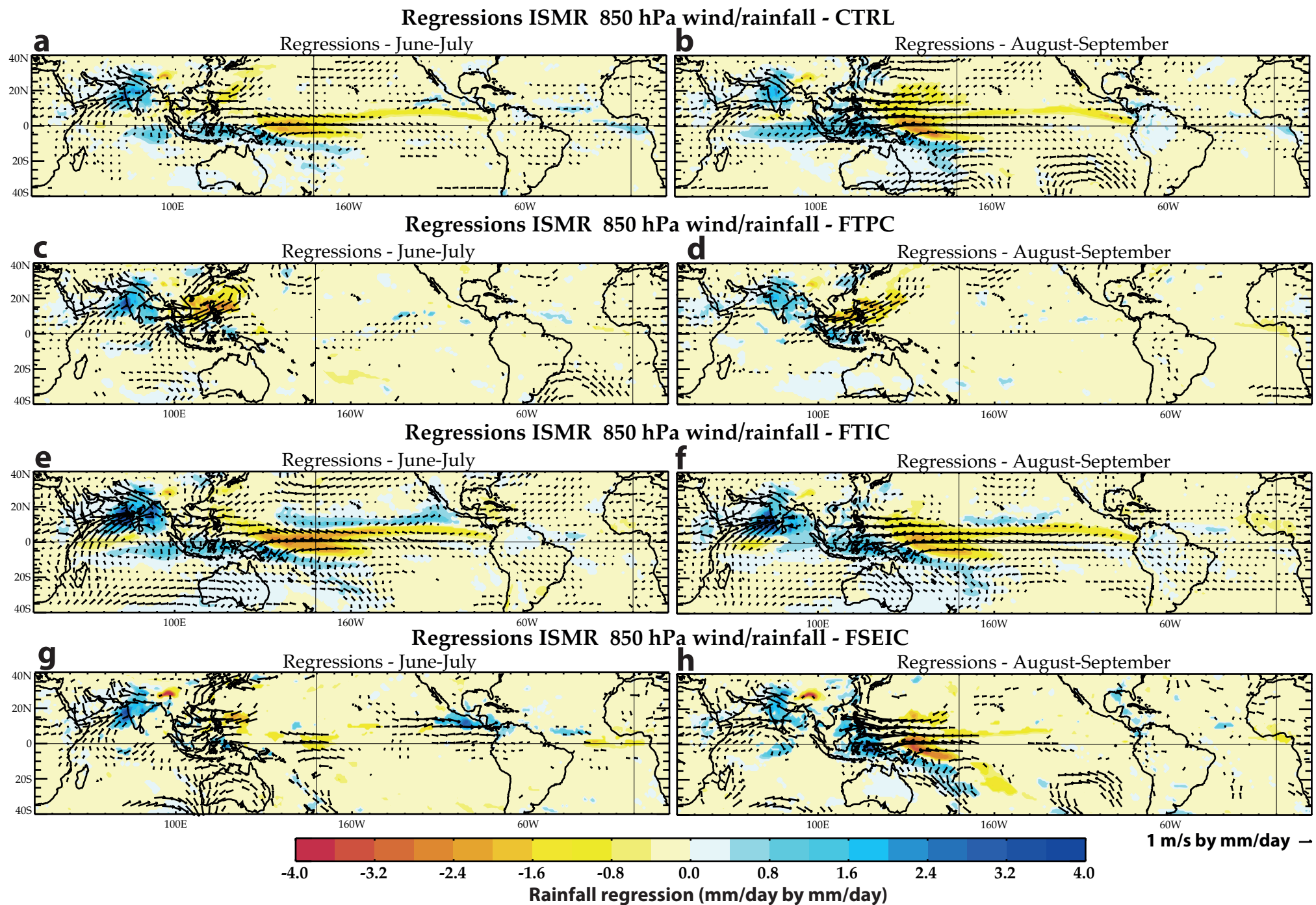
Figure 6: (a, b) June-July and August-September mean rainfall (shading) and 850-hPa wind (vectors) anomalies regressed against the ISMR index (e.g. JJAS ISM rainfall) in the CTRL experiment; (c, d) same as (a, b) but for the FTPC experiment; (e, f) same as (a, b) but for the FTIC experiment and (g, h) same as (a, b) but for the FSEIC experiment. Unit for the rainfall and 850-hPa wind regression coefficients are, respectively, in mm/day by mm/day and m/s by mm/day. Only rainfall and 850-hPa wind regression coefficients above the 95% significance confidence level according to a phase-scrambling bootstrap test (Ebisuzaki 1997) with 999 samples are shown.
