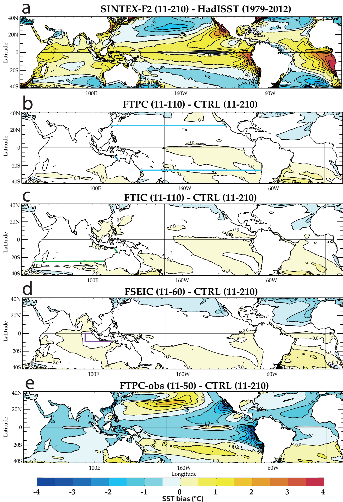
Figure 1: a) SST means difference ( ^{\circ}\text{C} ) between CTRL (years 11-210) and HadISST1.1 dataset (years 1979-2012); b) SST means difference ( ^{\circ}\text{C} ) between FTPC (years 11-110) and CTRL; c) SST means difference ( ^{\circ}\text{C} ) between FTIC (years 11-110) and CTRL; d) SST means difference ( ^{\circ}\text{C} ) between FSEIC (years 11-60) and CTRL and e) SST means difference ( ^{\circ}\text{C} ) between FTPC-obs (years 11-50) and CTRL. The nudging domains for FTPC, FTIC and FSEIC experiments are shown, respectively, in panels b (blue), c (green) and d (purple).
