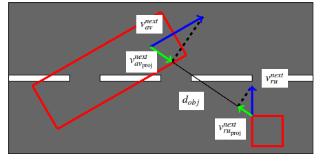
Fig. 3: Calculation of velocity projections
