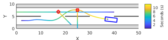
Fig. 10: Traj. for x_{veh}=40m , \theta_{ped}=\frac{3\pi}{4}rad for 5 transitions
