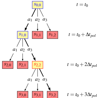
Fig. 4: Projection of future collision into previous states
