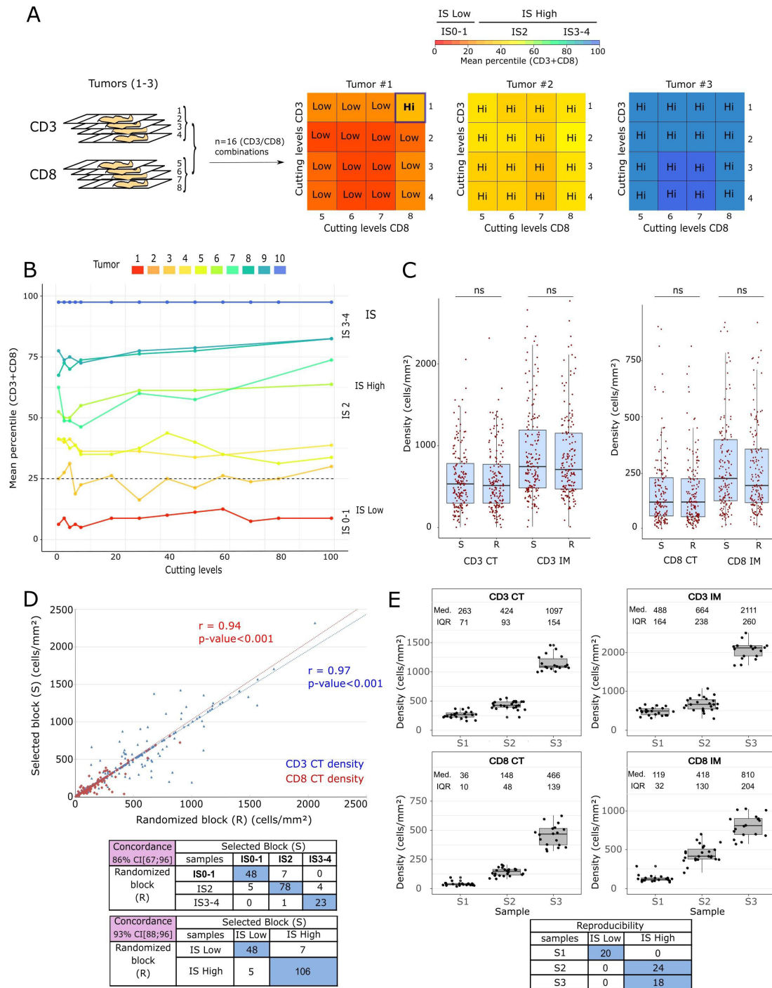
Figure 2 Analytical performance of the Immunoscore (IS). (A) Sample repeatability: assay stability in serial tumor sections. Impact of the selected sections on IS on three colon cancer samples according to the cutting level of the tumor block. For each tumor, four adjacent sections were immunostained for CD3+ followed by four adjacent sections immunostained for CD8+. All CD3+/CD8+ combination slides were tested per tumor. The concordance matrix shows the mean percentile (from red to blue; 0–100) of each combination (CD3+/CD8+) and the associated IS category. (B) Mean percentile (CD3+ and CD8+) and the IS variations according to the cutting level of the tumor block from top to bottom. A total of 13 levels (1, 3, 5, 7, 9, 20, 30, 40, 50, 60, 70, 80, 99) of cutting from 100 adjacent cuts of each tumor block (n=10) were investigated for IS. (C) Intermediate precision: impact of tumor blocks selection on the IS. Box plots show the IQR of CD3+ and CD8+ immune densities from the tumor block selected by the pathologist (S) and from a random block (R) for each patient of the cohort (n=166). Paired t-tests were calculated to assess differences between groups. (D) Pearson's correlation with r between densities in the randomized block and selected block for the CD3+ CT (blue) and CD8+ CT (red) (top). Contingency tables show the IS categories obtained for each case with the selected and random block (bottom). (E) IS assay precision and lot-to-lot reproducibility. Tumor cut from three colon cancers were assessed for CD3+ and CD8+ T cells densities using three different antibody lots, three DAB revelation kit lots, two Benchmark autostainers, three different runs and three operators. Contingency tables showing the IS classification concordance for each sample (bottom). CT, core of the tumor; IM, invasive margin.
