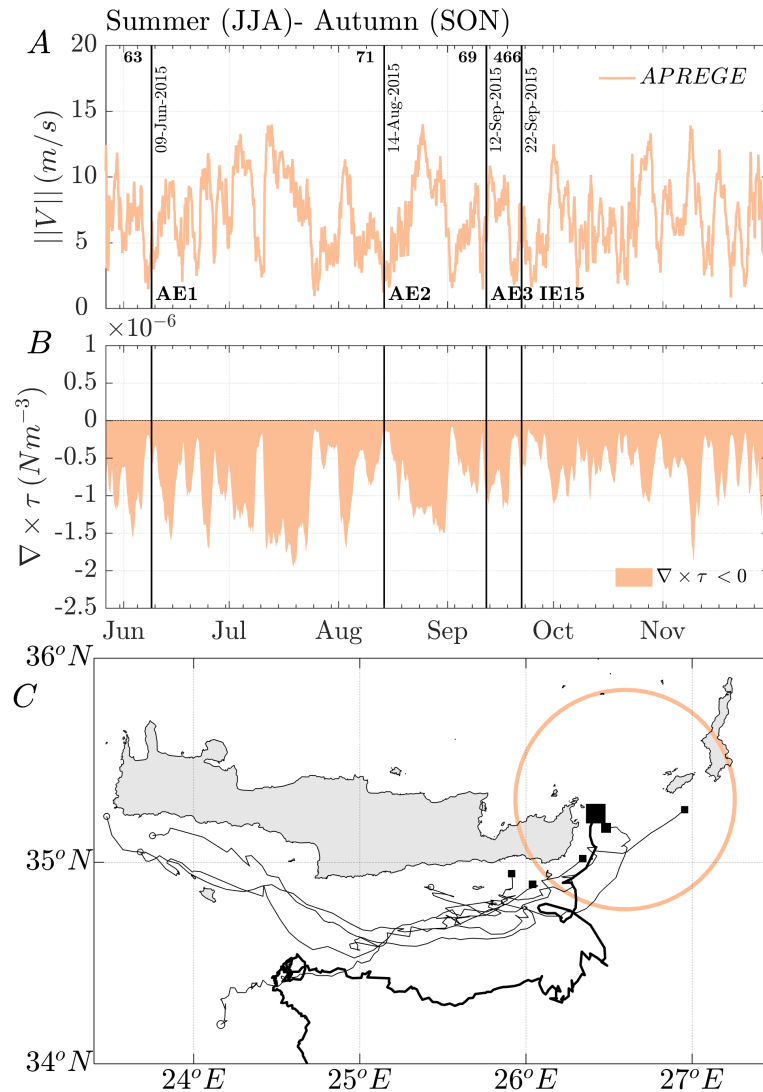
Figure 4. Time-series of A) wind speed ( m/s ) and B) negative wind stress curl \langle \nabla \times \tau \rangle are shown with the orange color as extracted from ARPEGE wind data. The selected area for analyzing the wind forcing climatology is illustrated with the orange circle in panel (C). Trajectories of long-lived ( > 2 weeks) eddies (gray colors) detected in CROCO model in the southeastern lee of Crete island during the summer & autumn of 2015. The first points of the eddy detection are plotted with the black square points while the points of last detection are illustrated with the open white circles. The longest-lived detected anticyclone is illustrated with the thick black line.
