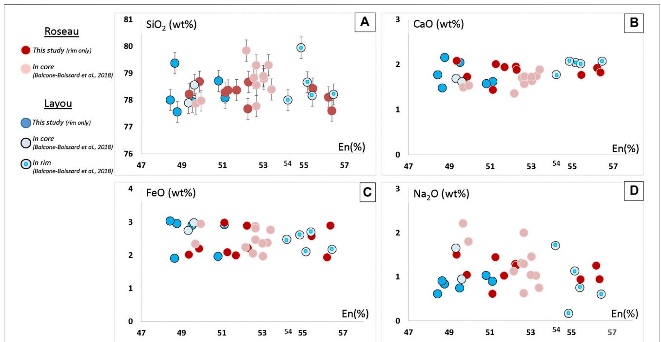
FIGURE 4 | Selected melt inclusion compositions as a function of host-orthopyroxene composition (En mol%). (A) SiO 2 ; (B) CaO; (C) FeO; (D) Na 2 O.
