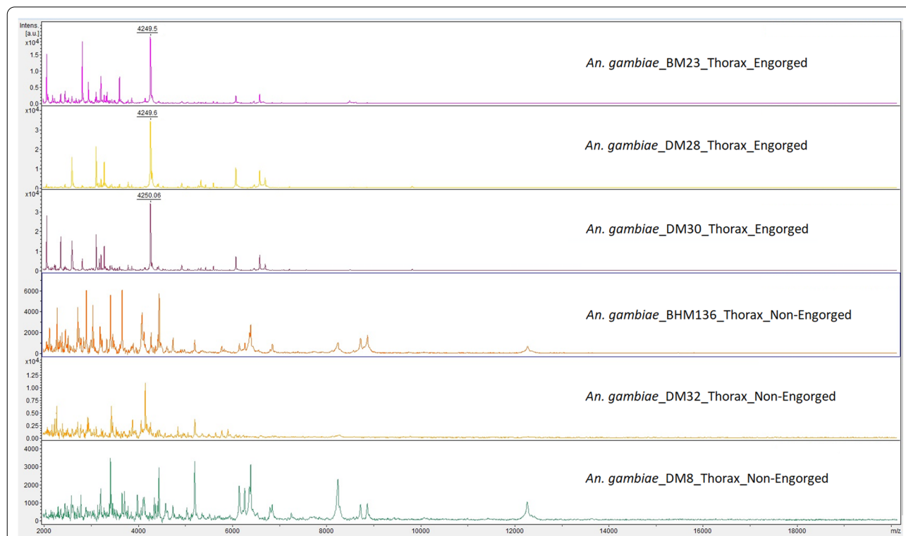
Fig. 5 Representative mass spectrum protein profiles of thorax from engorged and non-engorged Anopheles gambiae specimens of panel A from Mali. A.u arbitrary units, m/z mass to charge ratio in Daltons, F female
