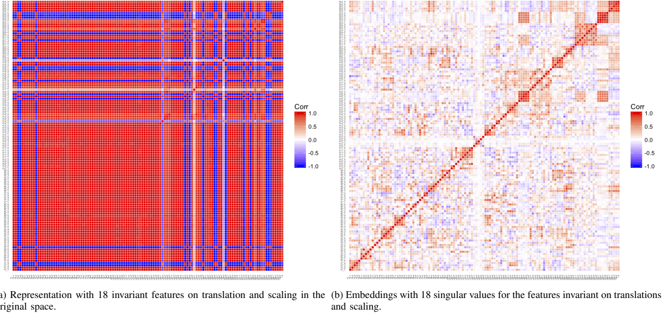
Fig. 3: Pearson correlation between BBOB instances.
