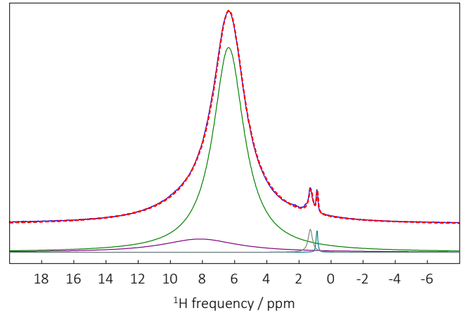
Figure 5. Experimental (blue) and fitted (red dashed line) ^1\text{H} MAS (60 kHz) NMR spectrum of H-titanate. The individual resonances used for the fit are shown below (see Table 1).
