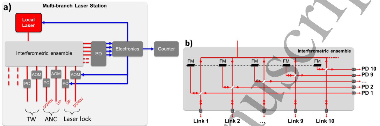
Figure 2 a) Schematic of a Multi-branch Laser station (PD=Photodiode, PC=Polarization Controller, AOM=Acousto-optic Modulator, TW=Two-Way, ANC=Active Noise Compensation). b) Schematic of the interferometric ensemble (FM=Faraday Mirror, PD=Photodiode).
