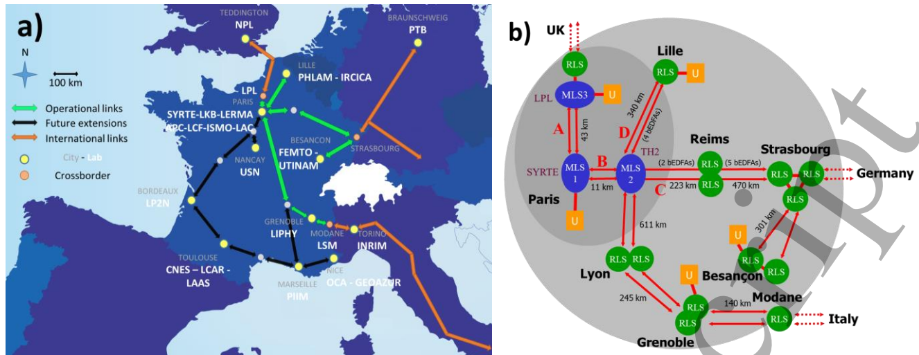
Figure 1 a) Current operational metrological network in France (REFIMEVE+ network) b) Sketch of the network architecture, MLS: multi-branch laser station, RLS: repeater laser station, bEDFA: bidirectional Erbium Doped Fibre Amplifier, U: user.
