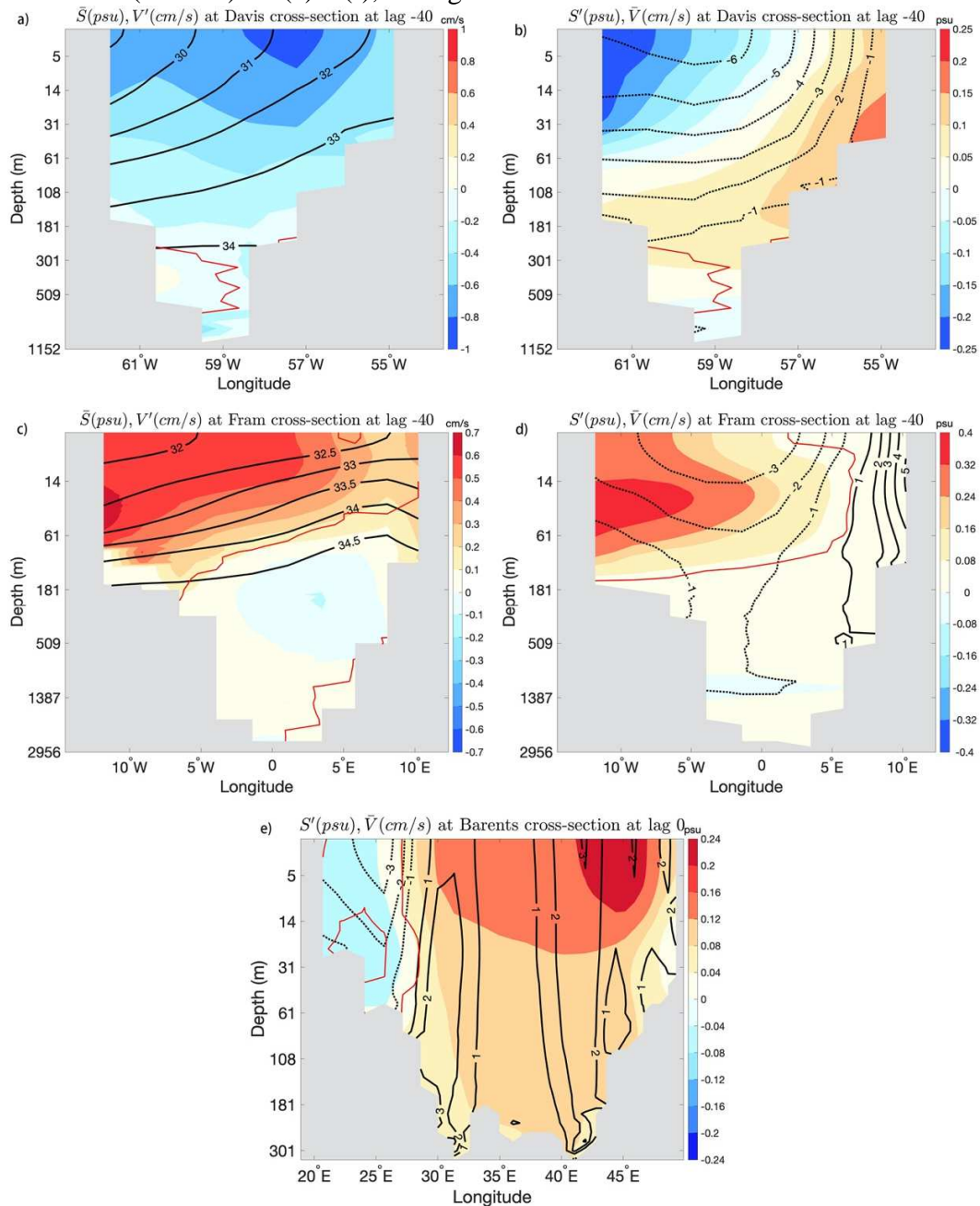
Figure 9. Salinity, in psu , and cross-section current, in cm \cdot s^{-1} at the Davis and Fram straits and Barents Sea Opening. (a) and (c) show the mean salinity (in black contours) and anomalous currents (in colors); (b), (d) and (e) show the mean currents (in black contours) and anomalous
