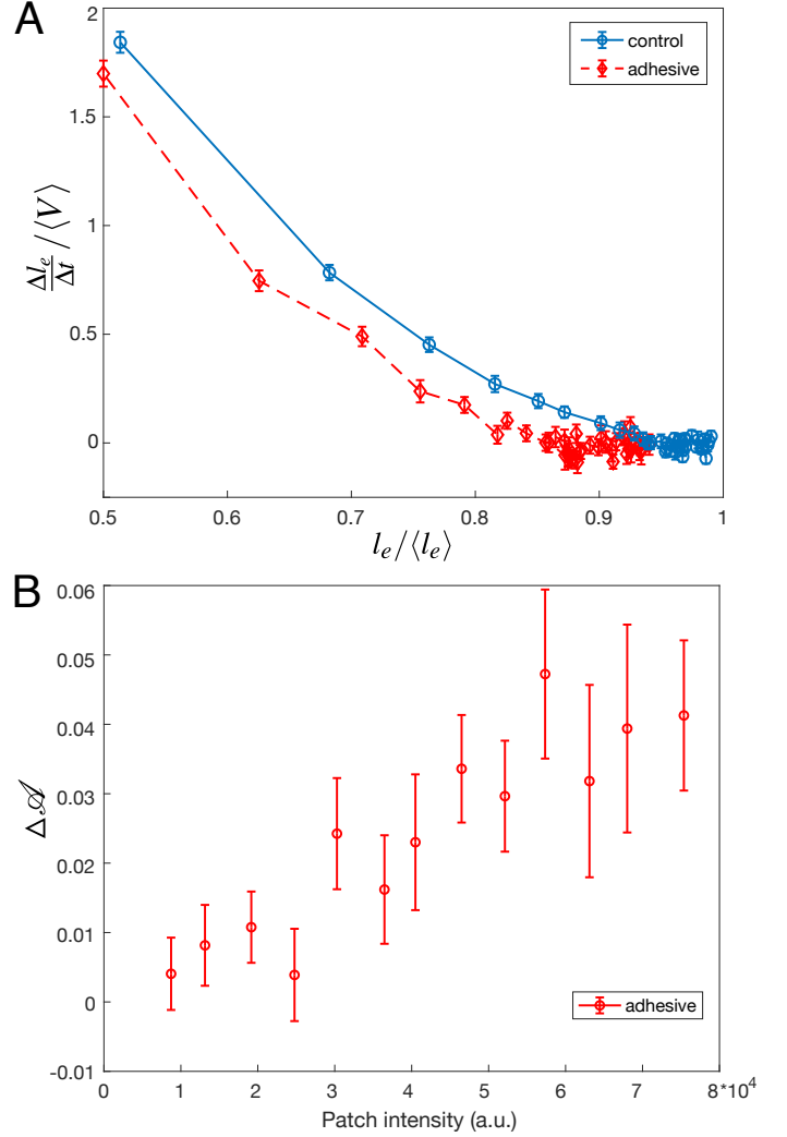
Fig. 4 Properties of individual rearrangements - (A) Rate of change of shrinking for dislocating edges of length l_e normalized by the average velocity of the flow \langle V \rangle plotted as a function of l_e normalized by the global average edges length \langle l_e \rangle . For a given l_e , a dislocating edge length is always disappearing more slowly for adhesive emulsions. (B) Difference in droplet deformation \Delta d before and after they undergo a T1 event as a function of adhesive patch intensity. An increase of patch intensity, i.e. an increase in binding energy, corresponds to higher values of droplet deformation accumulated before a T1 event.
