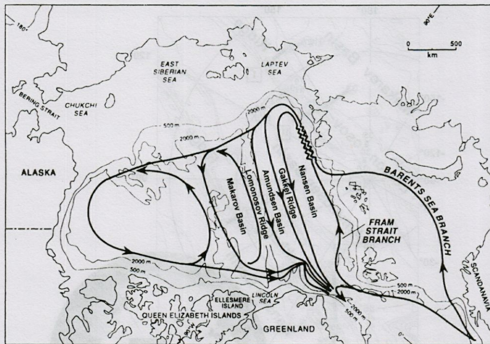
Fig. 2. – Circulation patterns of intermediate and deep waters (after Rudels et al. 1994).
