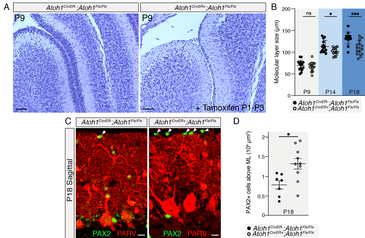
Figure S7: Depletion of granule cell precursors affects cerebellar development. Related to Figure 7.
