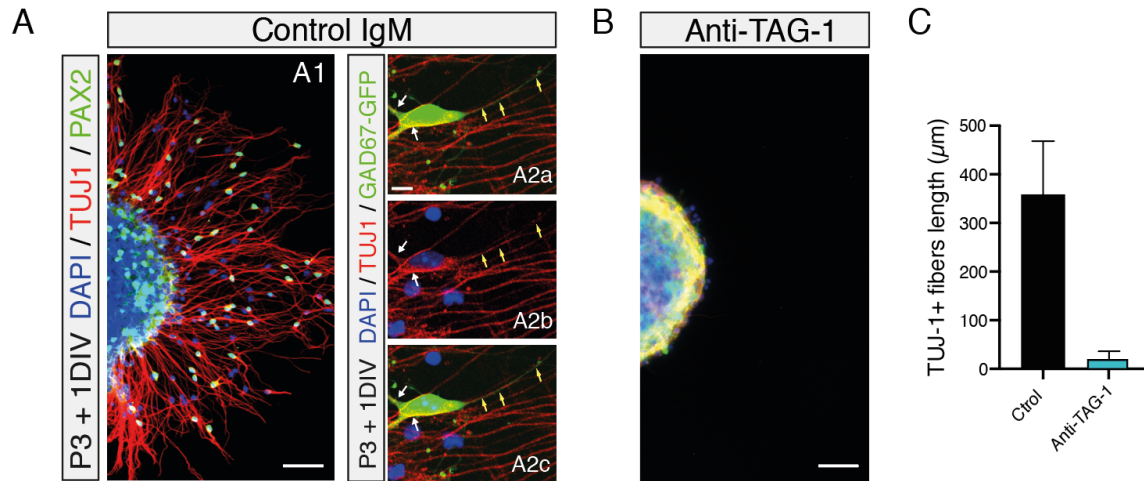
Figure S6: TAG-1 blocking antibody inhibits GC neurite outgrowth and MLGIs migration. Related to Figure 4 and Figure 5.
