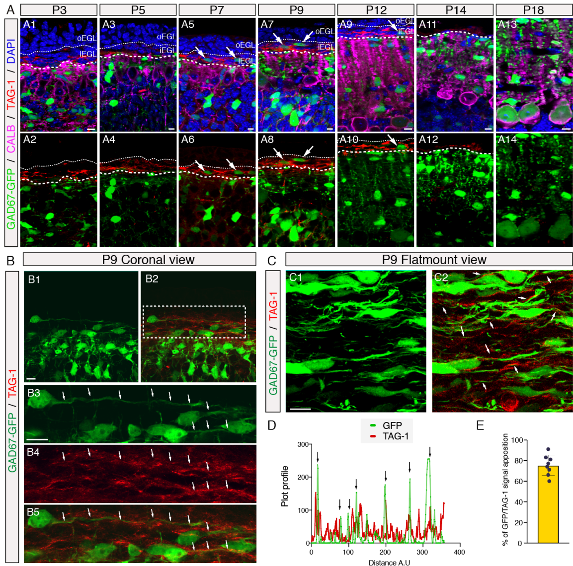
Figure S4: TAG-1 positive area delineates MLGI tangential migration territory. Related to Figure 3.
