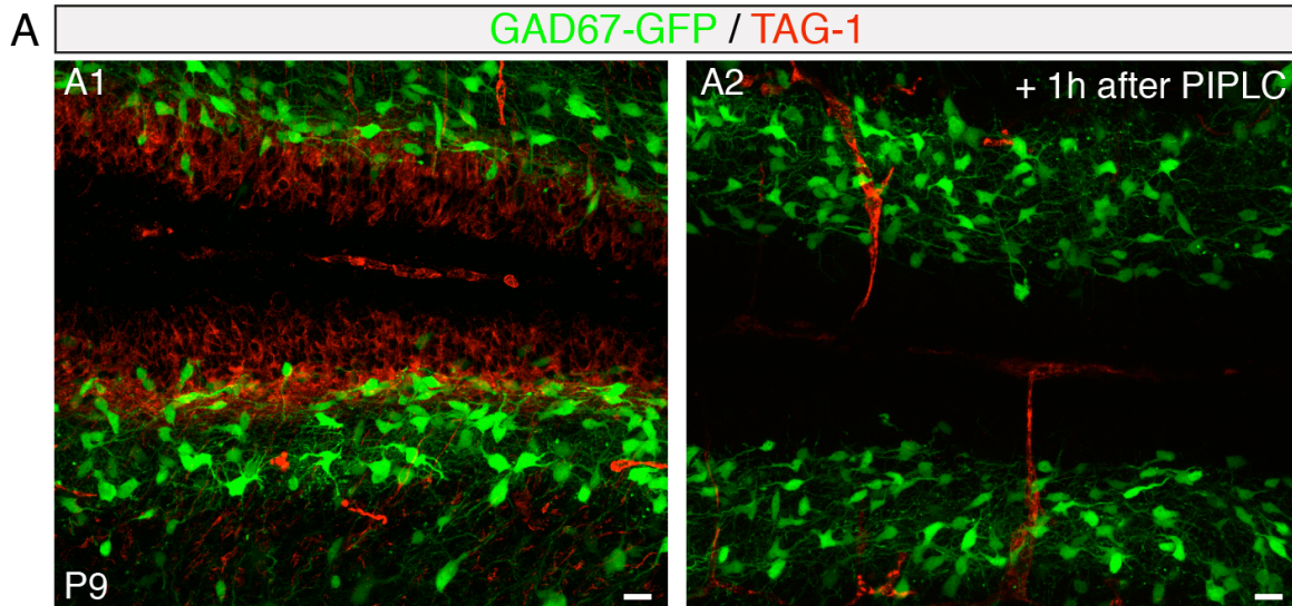
Figure S5: Acute treatment with PI-PLC completely removes TAG-1 expression in the EGL. Related to Figure 4.
