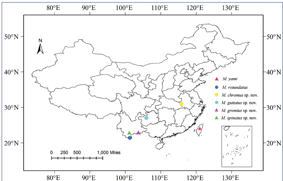
Figure 61. Geographic distributions of Metanigrus species.
