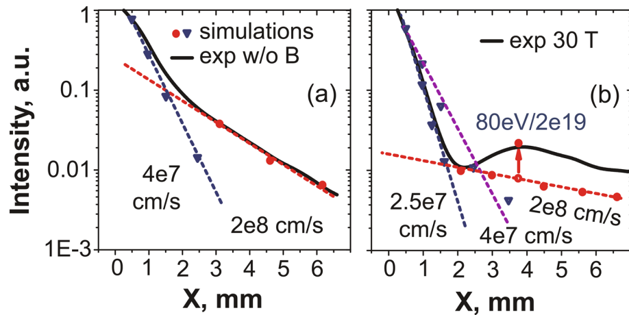
Figure 4. (a) Experimental (full) and simulated (dashed) spatial profiles of the X-ray resonance line Ly_\alpha in the free expansion case. The theoretical intensities were normalized by the corresponding experimental points. (b) Same in the case where a transverse magnetic field B = 30 T is applied. In the simulations, the excitation processes, as well as the recombination ones, were taken into account, as detailed in the “Methods” section. Note that the modelling, for the same velocity of the plasma component, but different densities can result in different slopes for the spectral intensity.
