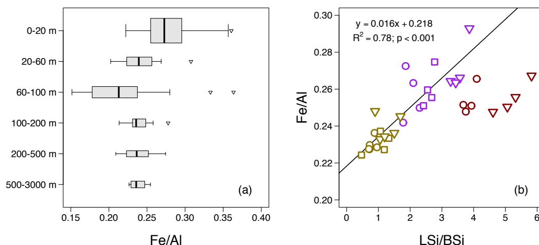
Figure 6: (a) Box whisker plot of the Fe/Al molar ratio ( \text{mol mol}^{-1} ) for suspended particles collected at TYR, ION, and FAST. The Fe/Al median values are 0.27 ( n = 37 ; 0-20 m), 0.24 ( n = 13 ; 20-60 m), 0.21 ( n = 17 ; 60-100 m), 0.24 ( n = 12 ; 100-200 m), 0.24 ( n = 9 ; 200-500 m), and 0.24 ( n = 10 ; 500-3000 m). For clarity, two outliers ( \text{Fe/Al} = 0.50 and 1.02 ) observed in the 0-20 m depth range are
