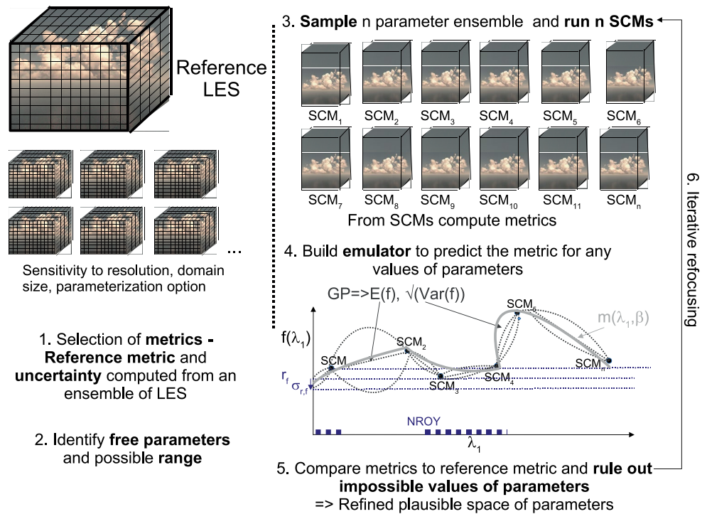
Figure 1. Schematic of the different steps of the htexplor tool.
