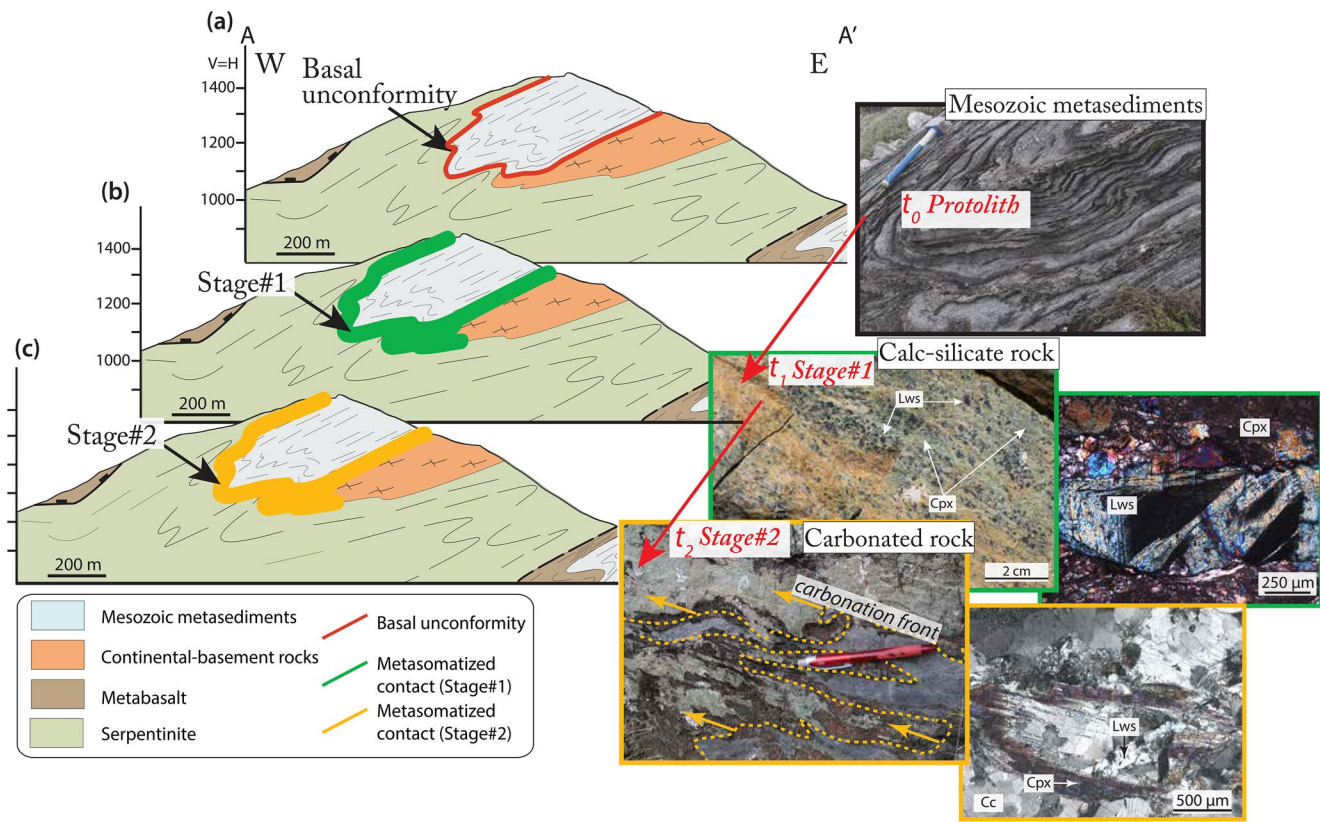
Figure 2. (a) Geological cross section along the A-A' profile of Figure 1b and field image of unaltered Mesozoic metasedimentary rocks. (b) Stage#1 metasomatism along the basal unconformity, field image and photomicrograph of the Stage#1 metasomatic rock (c) Stage#2 metasomatism superimposing on Stage#1 metasomatic rocks, field image showing the carbonation front replacing Stage#1 rock, and photomicrograph showing a replacement texture of Stage#1 assemblage by carbonate (Stage#2).
