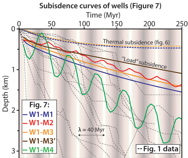
Fig. 8. Subsidence curves from different models in Figure 7 (wells W1-M1 to W1-M4) associated with Figure 1 bibliographic data. The subsidence of W1-M1, W1-M3 and W1-M3' is constant after 250 Myr ( i.e. still have a potential of subsidence), in contrast with the subsidence of W1-A1 and W1-A2 where it stops after 150 Myrs. The wells W1-M2 and W1-M4 show linear decay subsidence with deviations of different amplitude. See Figure 4B for the boundary conditions.
