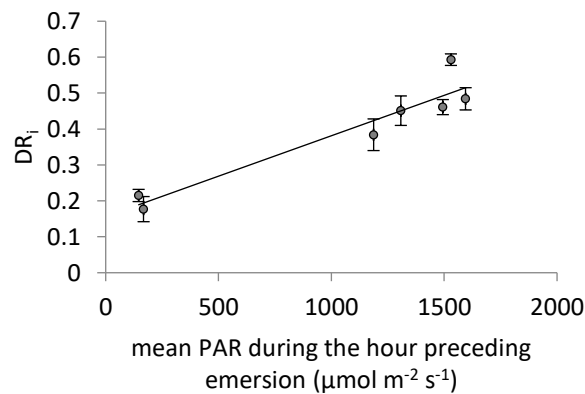
Appendix 2. Relationship between de-epoxidation ratio at the beginning of emersion ( \text{DR}_i , mean \pm se, n = 6 ) and the incident light during the hour preceding emersion (as mean photosynthetically available radiation, PAR, n = 60 )
