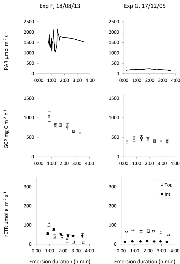
Figure 3. Incident light (as photosynthetically available radiation, PAR), gross community primary production (GCP, mean \pm se, n = 3), and relative electron transport rate (rETR, mean \pm se, n = 3) of thalli at the top and intermediate layers of the Fucus serratus canopy measured over emersion on different dates
