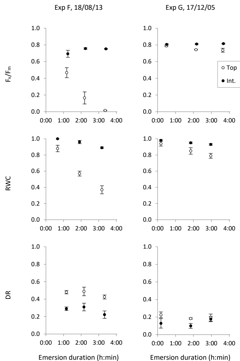
Figure 5. Mean ( \pm se, n = 3 ) optimal quantum yield of PSII ( F_v/F_m ), relative water content (RWC) and de-epoxidation ratio (DR) measured during emersion on thalli at the top and intermediate layers of the Fucus serratus canopy on different dates
