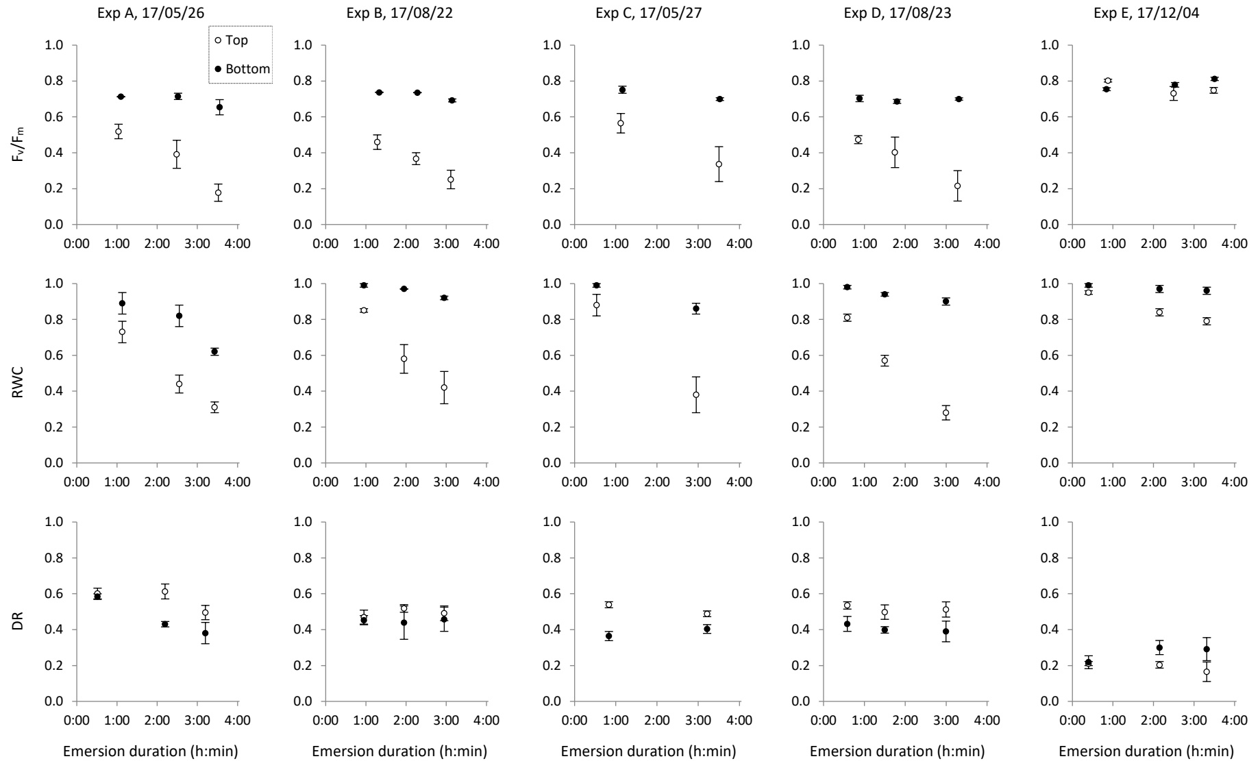
Figure 4. Mean ( \pm se, n = 3 ) optimal quantum yield of PSII ( F_v/F_m ), relative water content (RWC), and de-epoxidation ratio (DR) measured during emersion on thalli at the top and bottom of the Fucus serratus canopy on different dates
