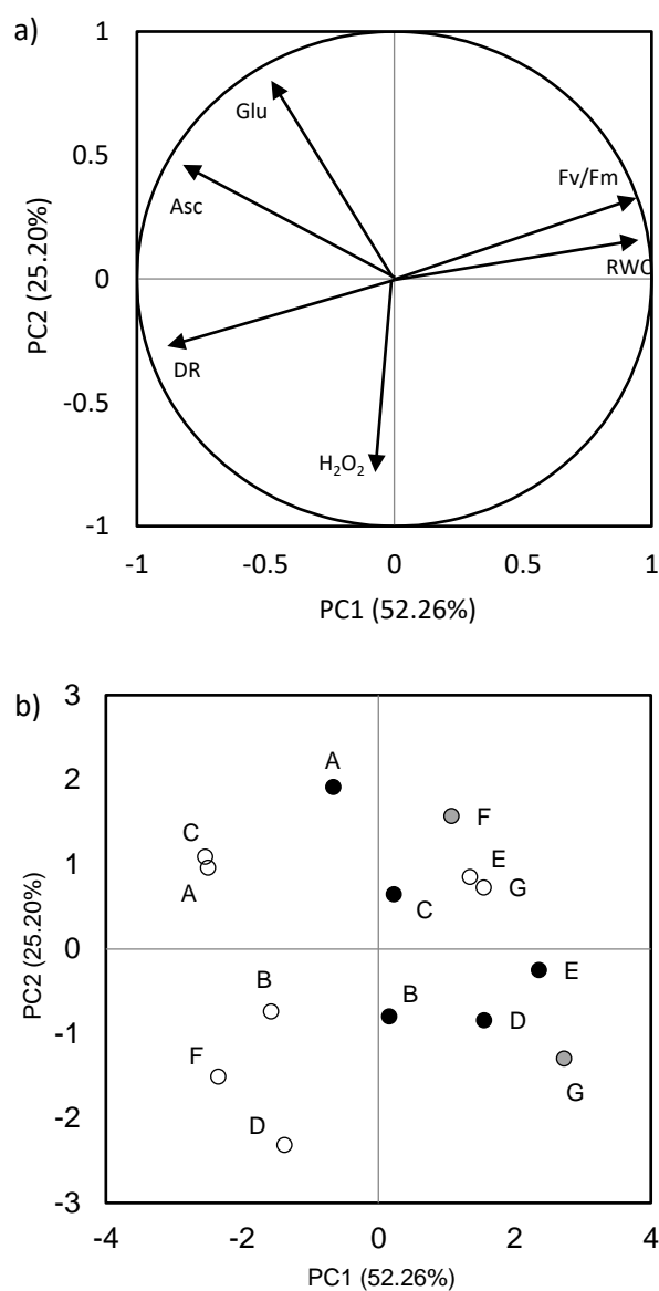
Figure 6. Projection onto the PC1-PC2 plane (a. Variables map, b. Objects map) of the results of principal component analysis (PCA) performed on the mean values of biochemical parameters (de-epoxidation ratio (DR), hydrogen peroxide ( H_2O_2 ), ascorbate (Asc), and glutathione (Glu) contents), relative water content (RWC), and optimal quantum yield ( F_v/F_m ) measured at the end of the emersion period on May (A, C), August (B, D, F) and December (E, G) in thalli from different layers of the Fucus serratus canopy: top (white), bottom (dark) and intermediate (grey)
