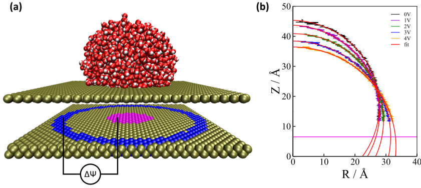
FIG. 2: (a) Representation of the electrowetting-on-dielectric simulated system. Ochre atoms below the aqueous drop constitute a hydrophobic insulator monolayer. The magenta and blue atoms are the inner and outer platinum electrodes, which are also separated by an insulator ring (a vertical shift was introduced between the two layers of the substrate material for a better visualization). (b) Vertical cross section of the water droplet on the insulator surface at various applied voltages. The contact angle is determined by a fit of the drop contour. Adapted with permission from Ref. [3], ACS Nano 2016, 10 , 8536, Copyright (2016) American Chemical Society.
