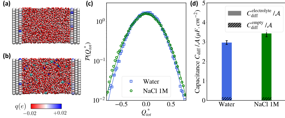
FIG. 1: Capacitors consisting of graphite electrodes separated by (a) pure water and (b) a 1M aqueous NaCl solution under a voltage \Delta\Psi = 0 V; the color bar indicates the instantaneous charge of the electrode atoms. (c) Distribution of the total charge of the electrode Q_{tot}^* for both systems, computed within Born-Oppenheimer dynamics simulations; solid lines are normalized Gaussian distributions with the corresponding standard deviation. (d) Contributions to the differential capacitance per unit area C_{diff}/A at 0 V: from the empty capacitor, C_{diff}^{empty}/A , and from the charge fluctuations induced by the electrolyte, C_{diff}^{electrolyte} = \beta \langle \delta Q_{tot}^{*2} \rangle (see Eq. 5 of the main text); the latter corresponds to the variance of the distributions of panel (c). Panels a, b and d adapted from Ref. [1], Phys. Chem. Chem. Phys. , 2020, 22 , 10480 by permission of the PCCP Owner Societies.
