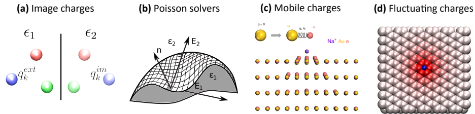
FIG. 1: Strategies to account for the polarization of the metal by the electrolyte in molecular simulations. (a) Image charges q_k^{im} inside the solid with permittivity \epsilon_2 induced by the electrolyte charges q_k^{ext} in a medium of permittivity \epsilon_1 (see Eq. 1). (b) Solving the Poisson equation on a grid to compute the induced (surface) charges. (c) Describing the electronic response with mobile charges: here gold atoms are modeled using opposite charges tethered by a spring, with the cores representing the nuclei (yellow) fixed and the shells (pink) moving in response to the presence of a sodium ion (purple). (d) Describing the electronic response with fixed sites with fluctuating charges: here the charge of atoms in a graphite electrode is distributed inhomogeneously (darker red means more negative) in response to the presence of a cation such as \text{Li}^+ (blue). Panel b reproduced from Ref. [42], J. Chem. Phys. 2010, 132 , 154112, with the permission of AIP Publishing; panel c reproduced from Ref. [45], Nature Commun. 2018, 9 , 716, with permission of Springer Nature.
