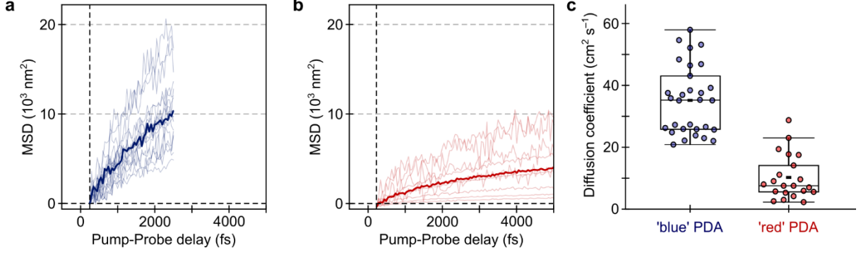
Figure 2: Femtosecond transient absorption microscopy results for ‘blue’ and ‘red’ PDA. a-b. MSD curves for ‘blue’ (a) and ‘red’ PDA (b), respectively. Solid line shows average curves whereas faint lines are from individual sample locations. Due to the faster decay in ‘blue’ PDA, the MSD was only recorded to 2.3 ps. c. Scatter-box plot of diffusion coefficients for ‘blue’ and ‘red’ PDA. Boxed area is 25-75% range, with horizontal line representing median and whiskers for interquartile range. Filled black rectangles represent the mean.
