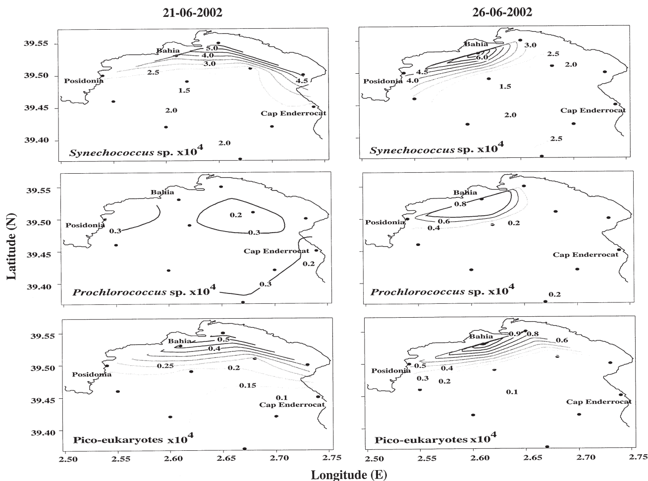
Fig. 3. – Distribution of Synechococcus sp., Prochlorococcus sp. and pico-eukaryotes cell abundance (cells ml -1 × 10 4 ) at the surface waters of the Bay of Palma, during two sampling surveys in June 2002. Full circles: sampling stations.
