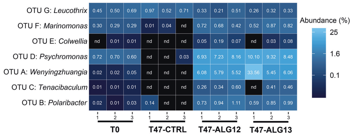
Fig. 5 Heatmap of the relative sequence abundance of 13 C-incorporating OTUs in the total communities based on 16S rRNA gene metabarcoding of non-fractionated DNA. Triplicates of the different conditions are shown in separate columns. nd not detected.
